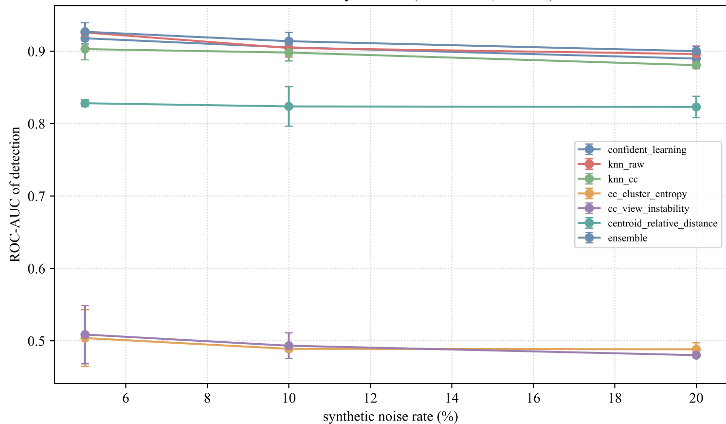
Noise detection by method (mean \pm std, 2 seeds)
