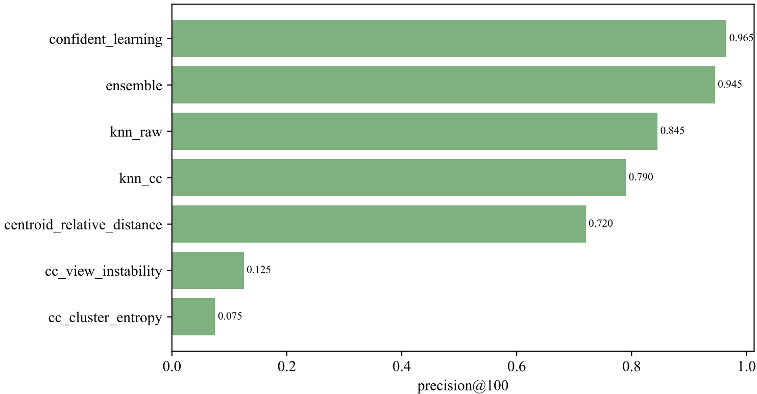
Noise detection — precision@100 at 10% synthetic noise
