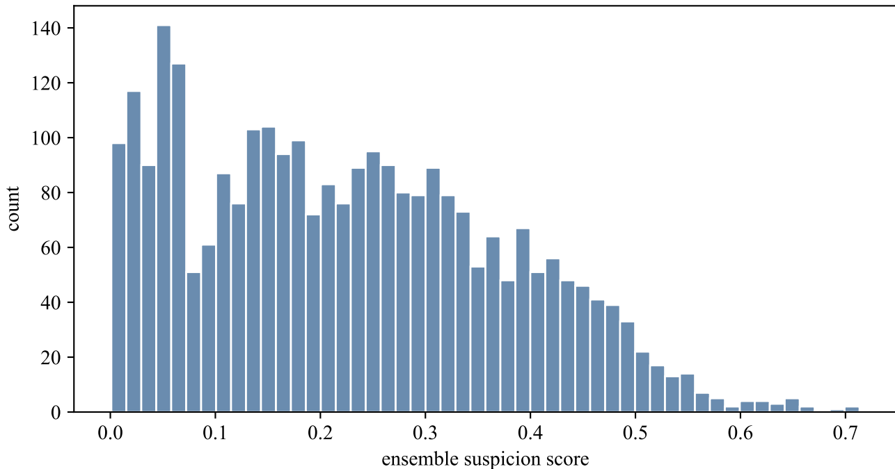
Distribution of ensemble suspicion scores (real data) — long right tail = candidates
