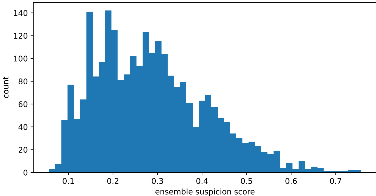
Distribution of ensemble suspicion scores (real data)
