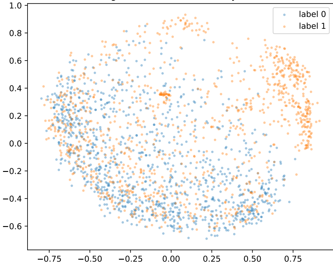
CC embeddings — PCA 2D (coloured by observed label)
