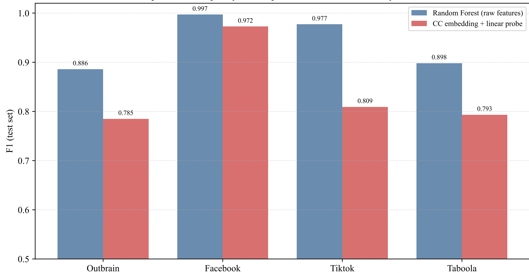
Representation quality — CC probe vs Random Forest, by source
