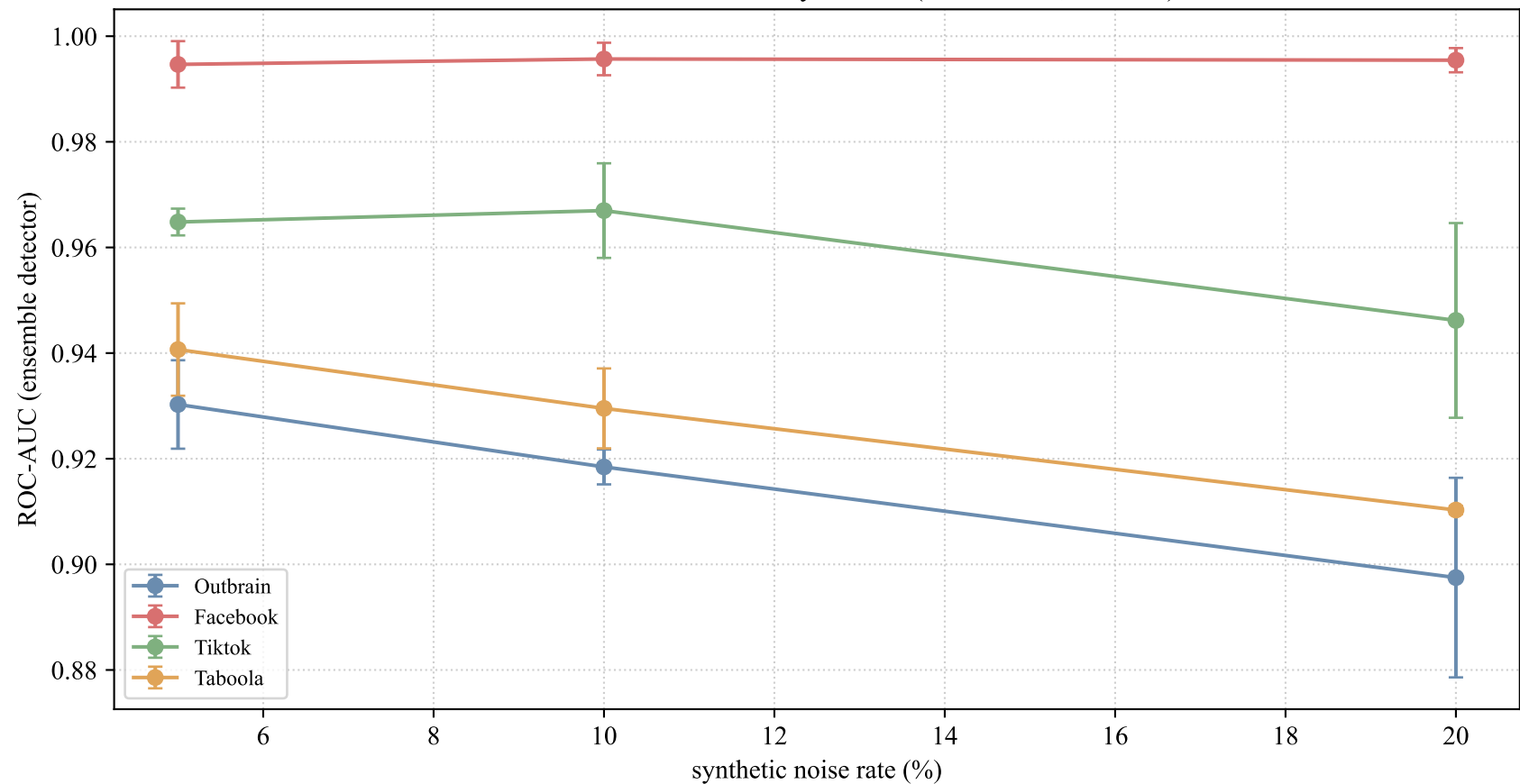
Ensemble noise detection by source (mean \pm std, 2 seeds)
