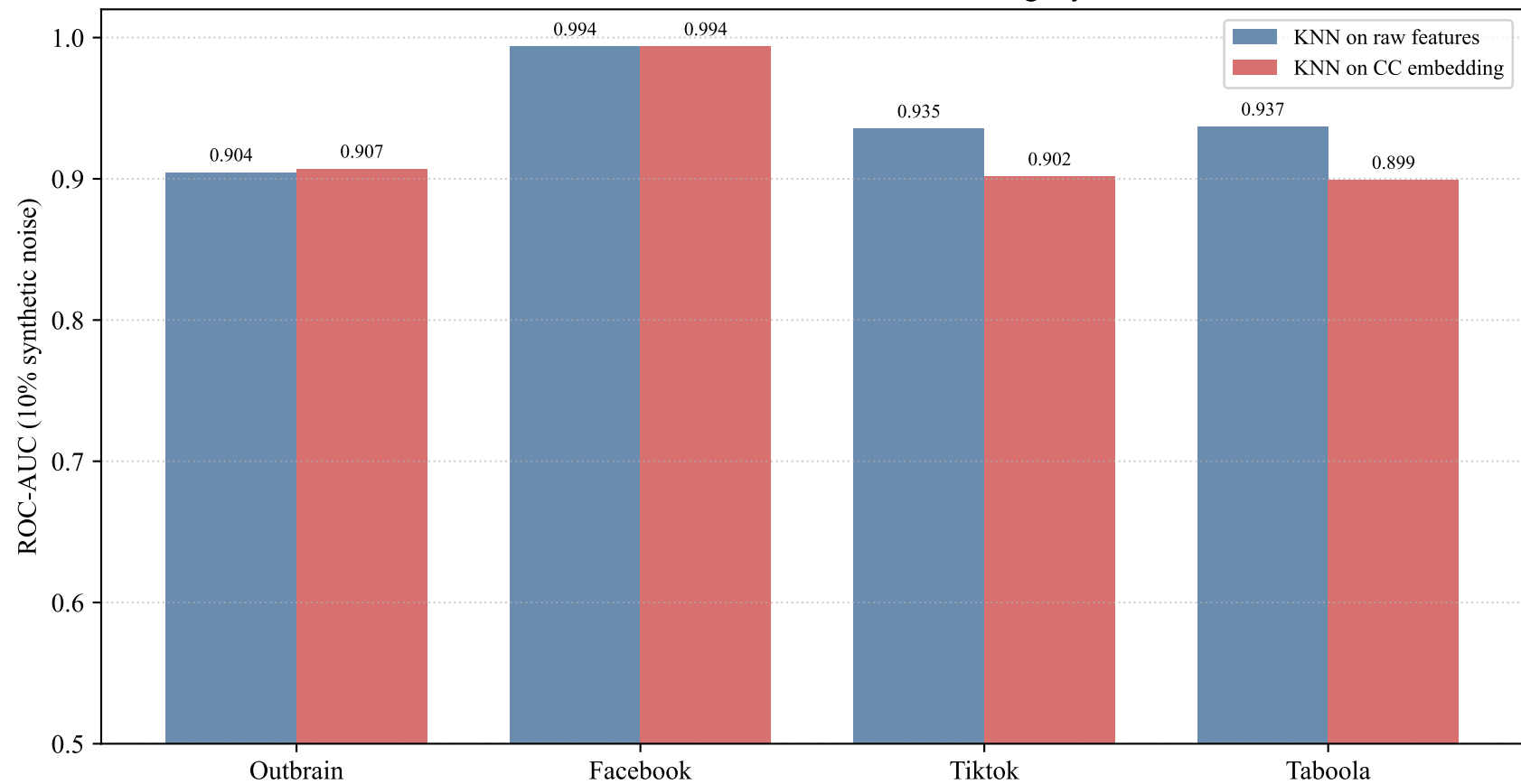
KNN noise detection — raw vs CC embedding, by source
