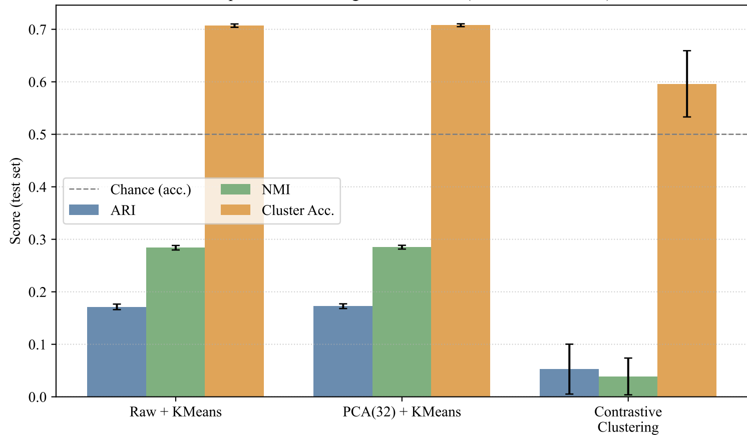
Unsupervised clustering vs. true labels (mean \pm std, 3 seeds)
