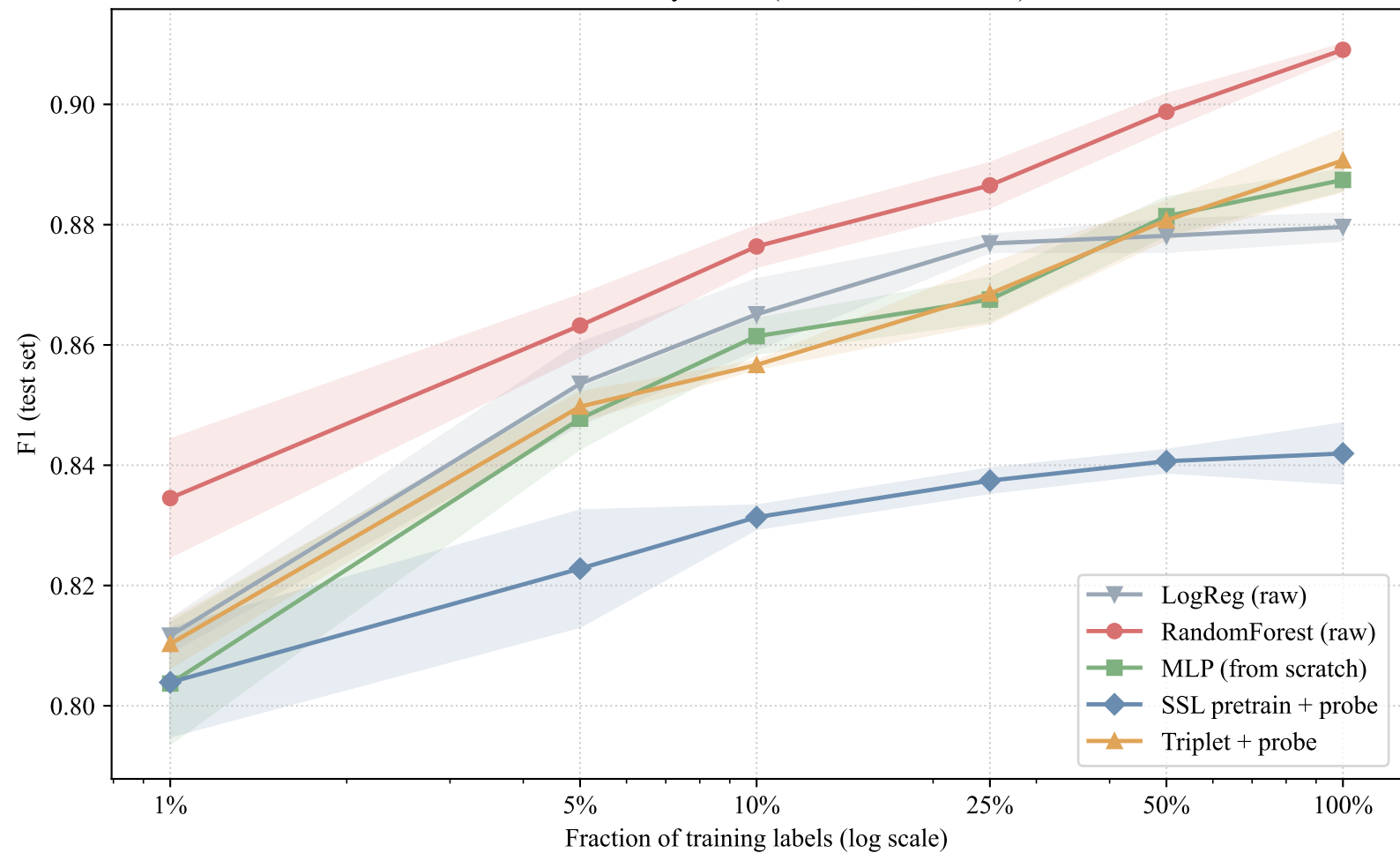
Label-efficiency curve (mean \pm std, 3 seeds)
