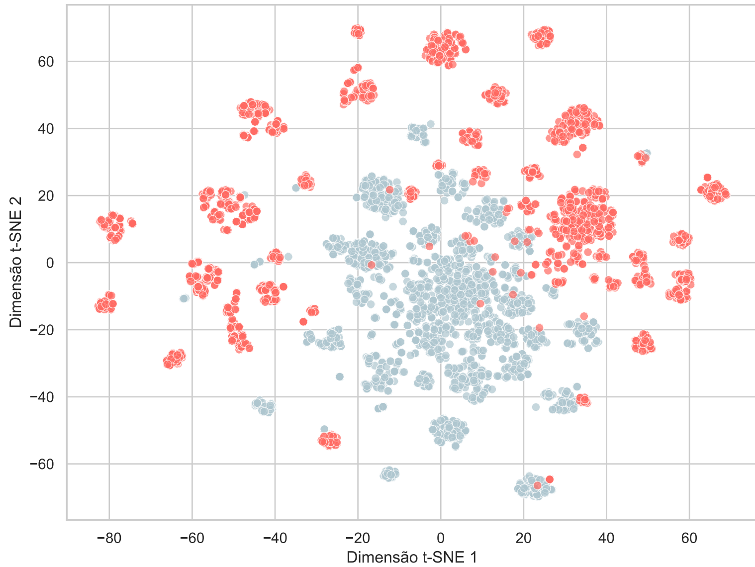
Raw Features
