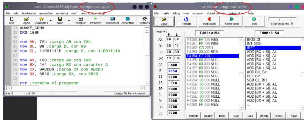
Figura 1: program1.asm
