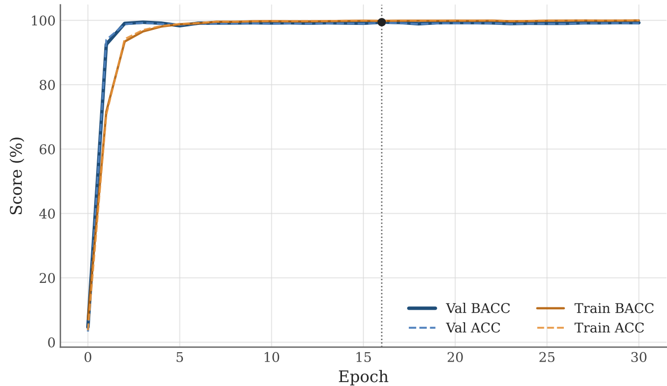
ResNet18 OrganCMNIST Training Curve
