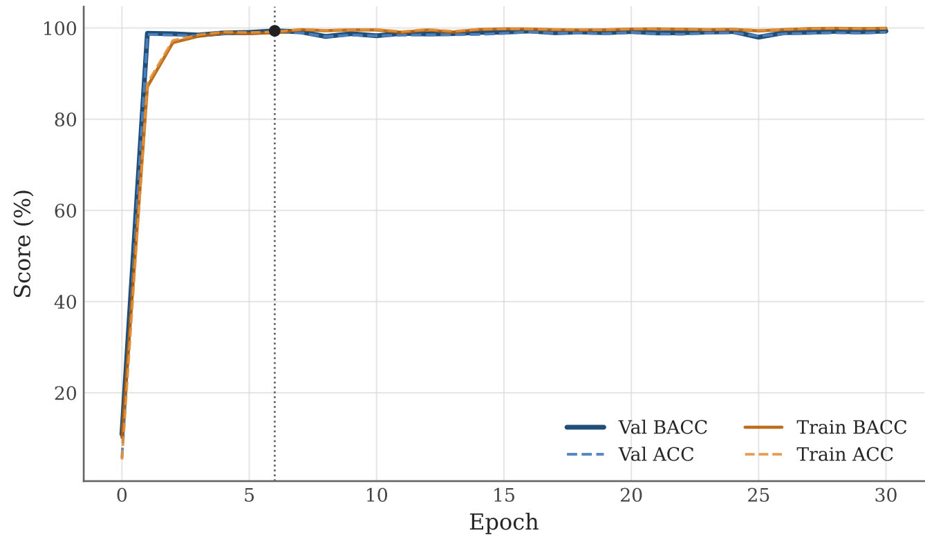
ResNet34 OrganCMNIST Training Curve
