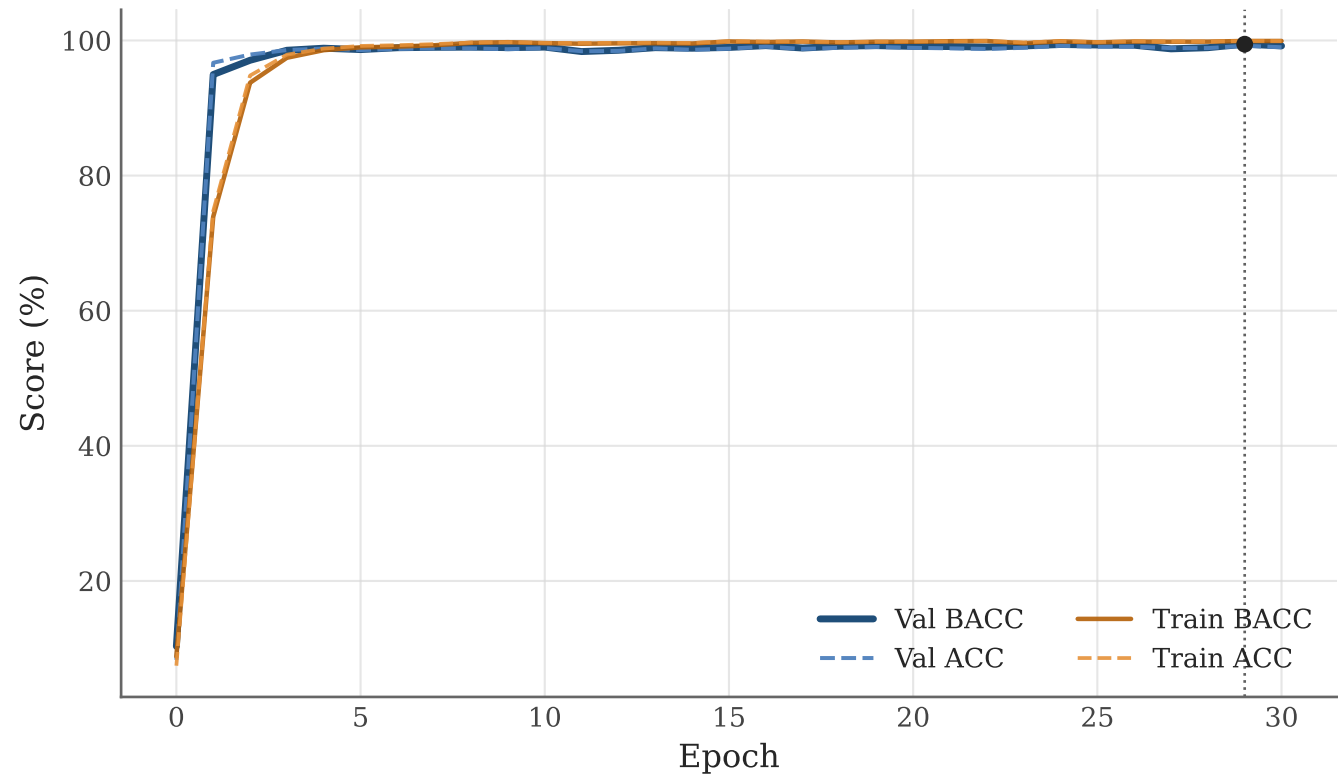
ResNeXt50 OrganCMNIST Training Curve
