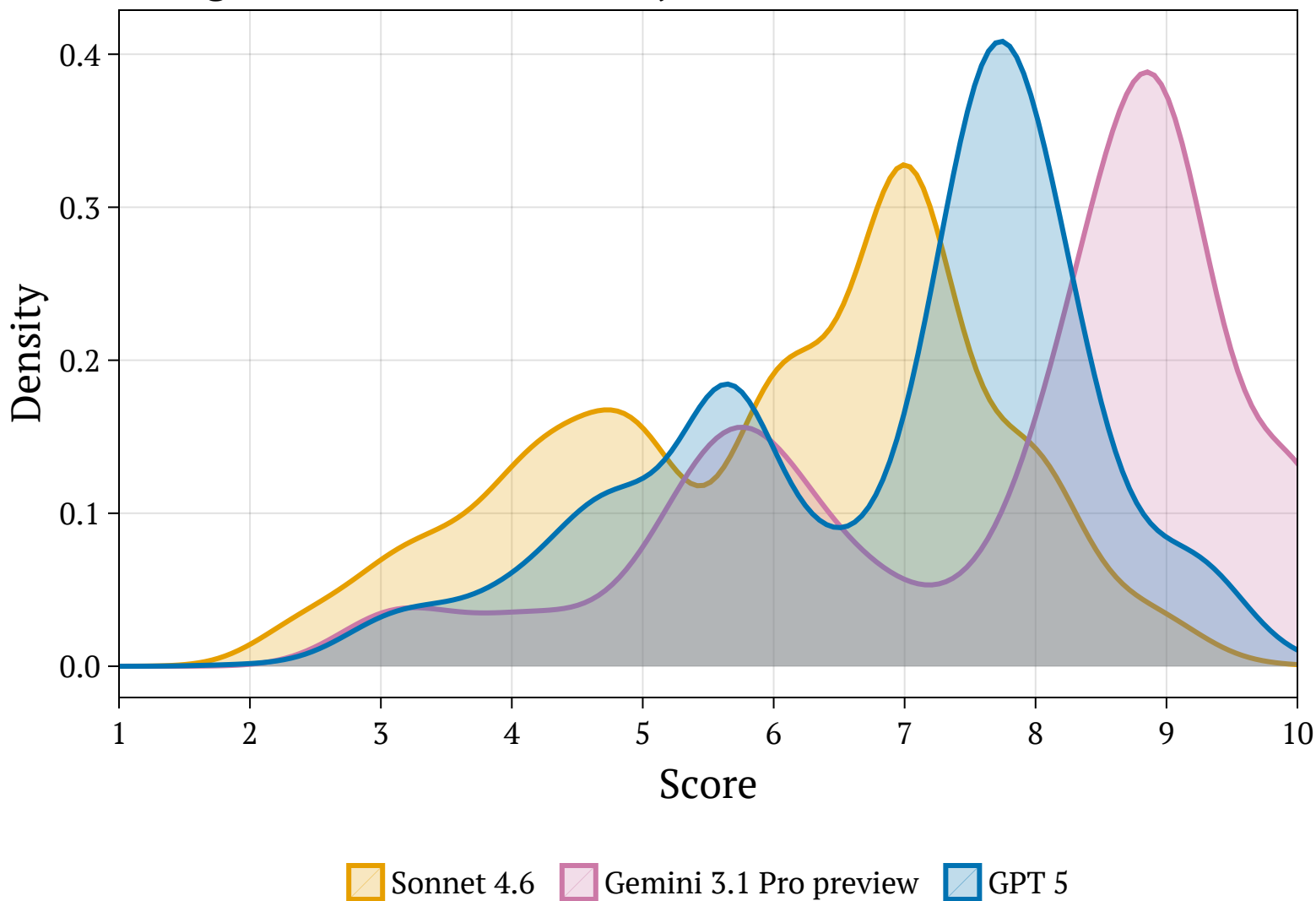
Cs Bigram score distribution by LLM
