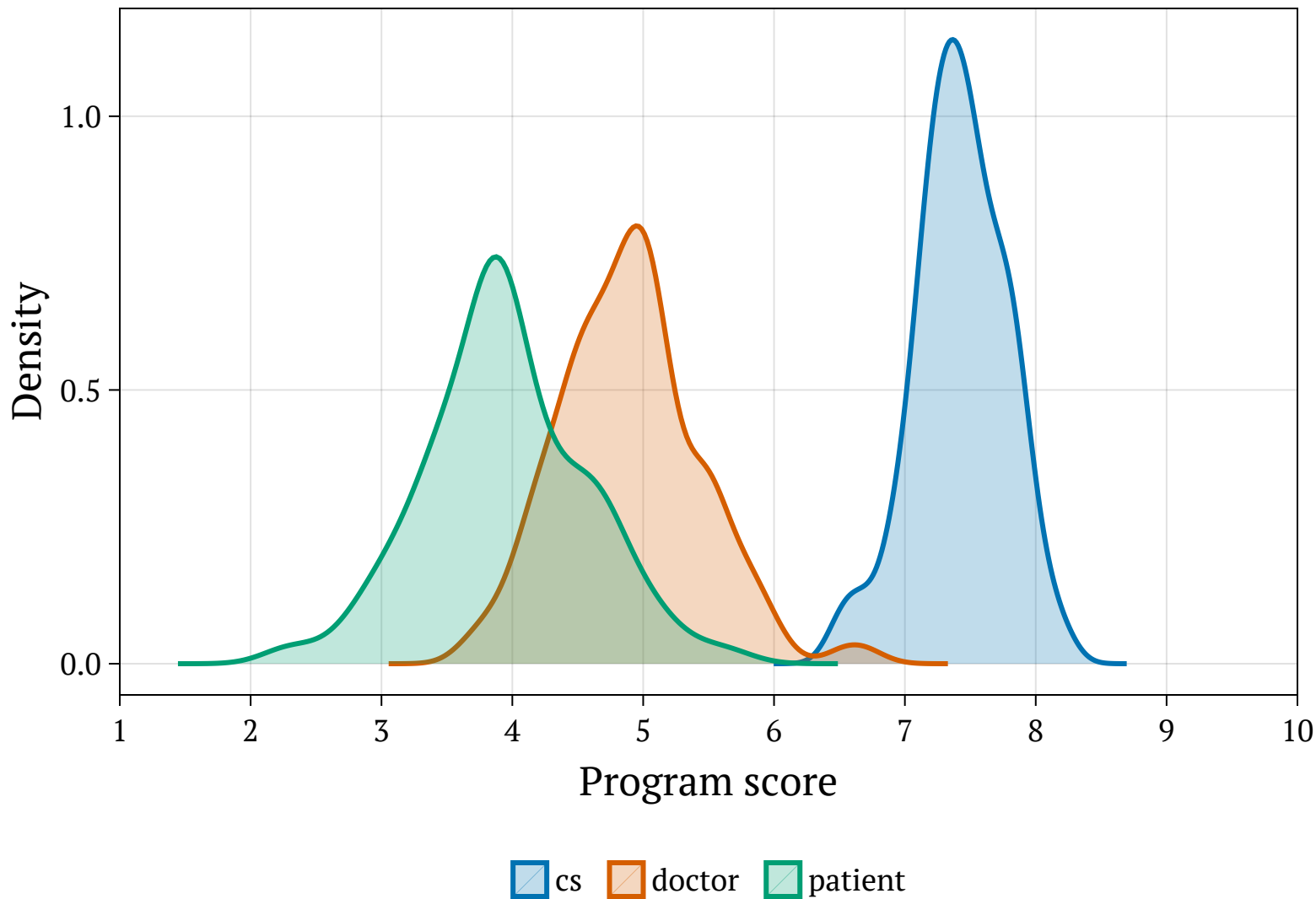
Program mean bigram score distribution by audience
