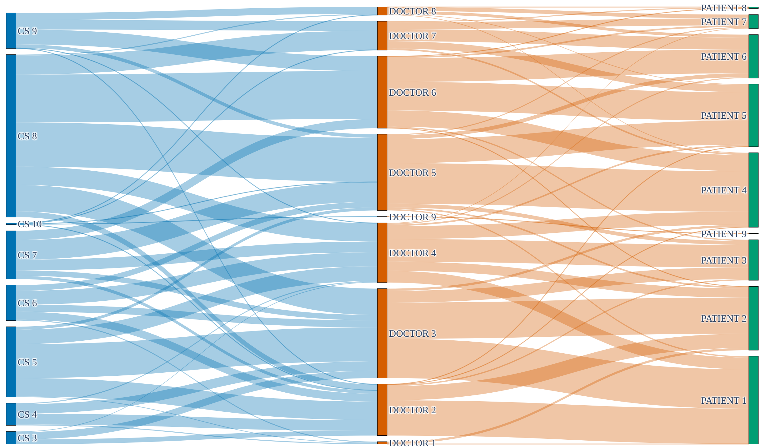
Global Bigram score flow: CS → Doctor → Patient
