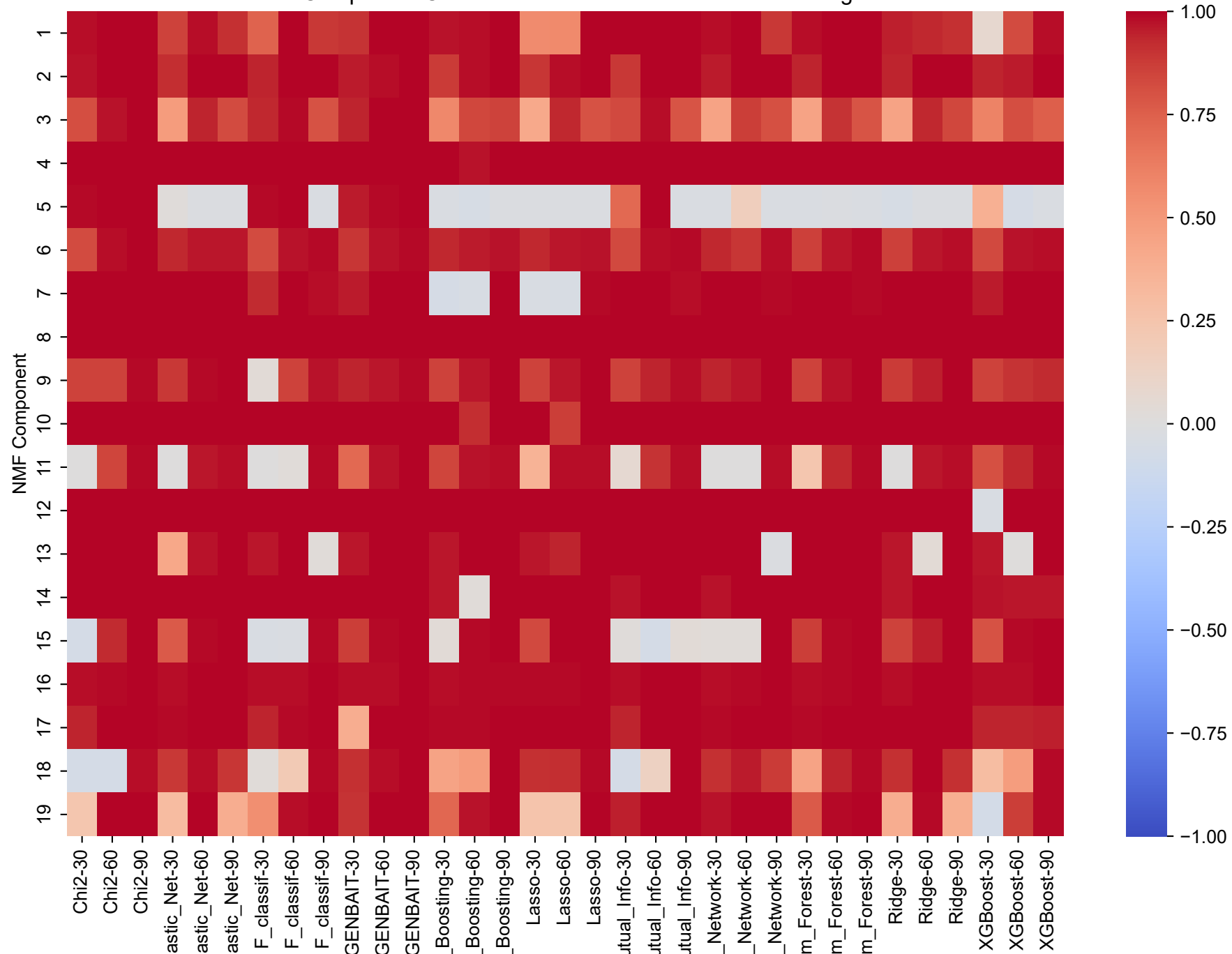
NMF Component Correlations Across Methods and Bait Lengths
