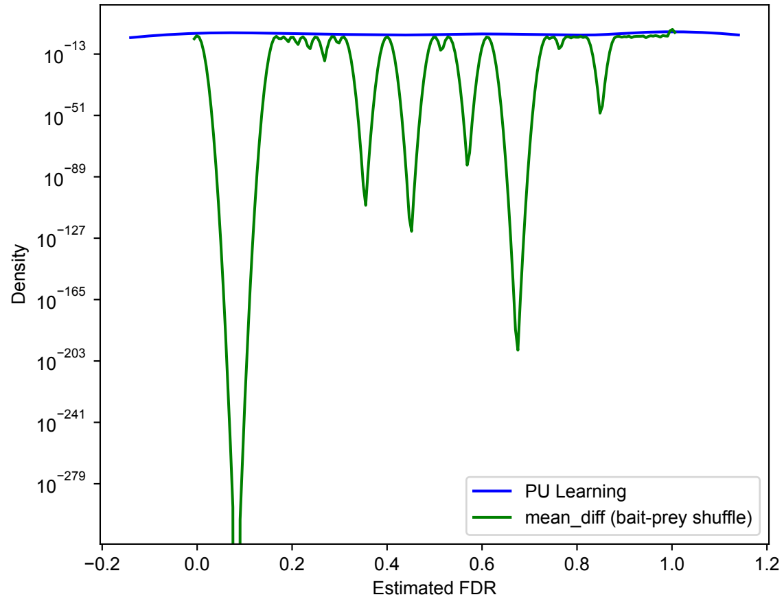
Density Plot of Assigned FDRs
