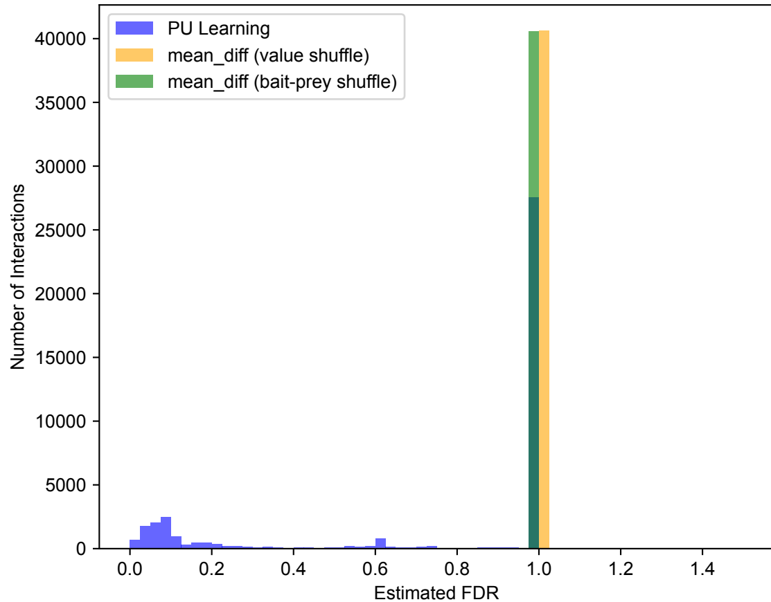
Histogram of Assigned FDRs
