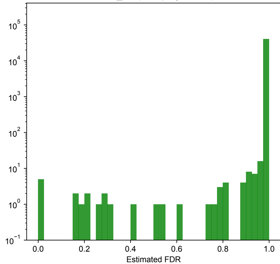
mean_diff (bait-prey shuffle)
