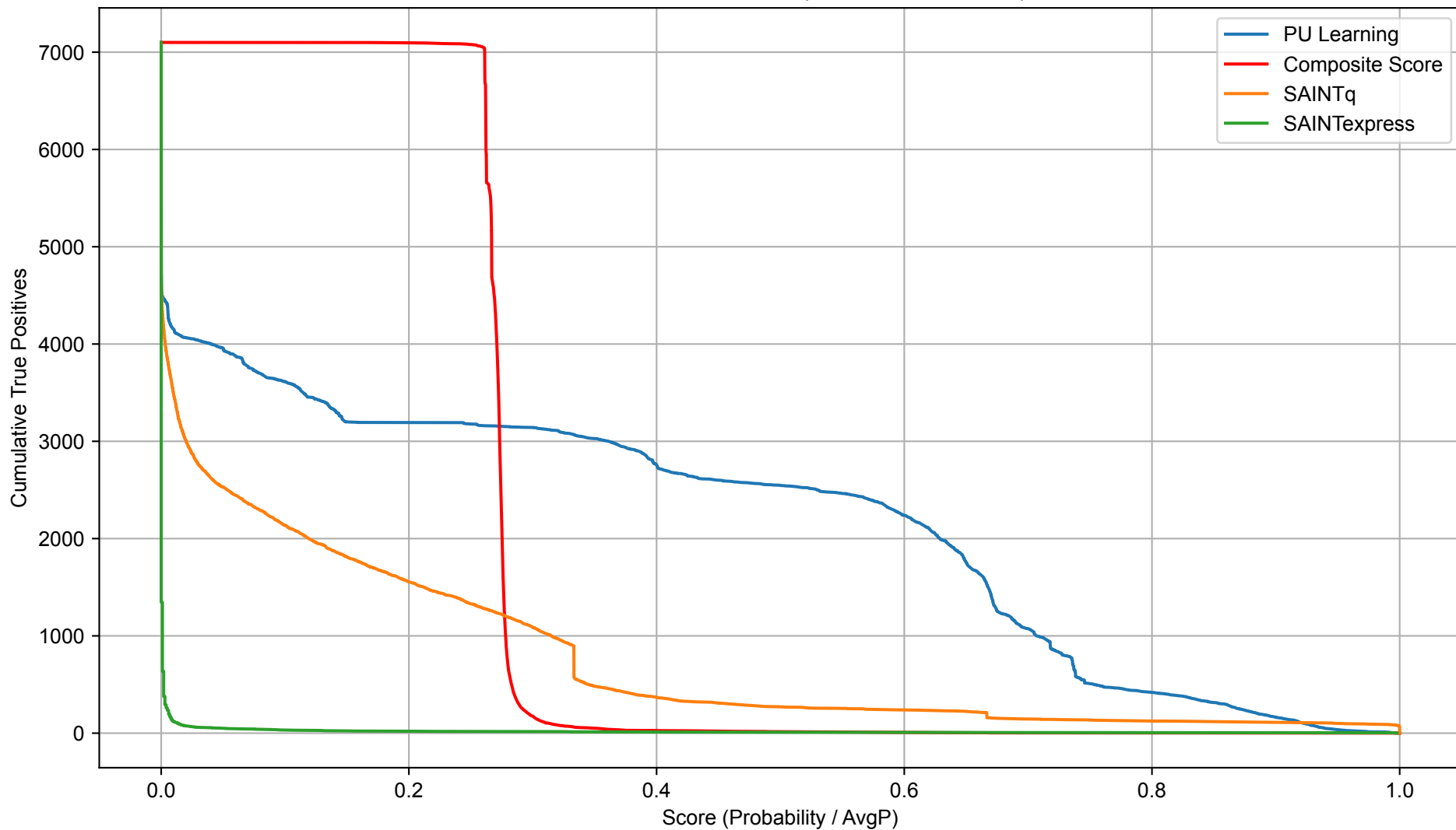
True Positives vs Score (All Baits Combined)
