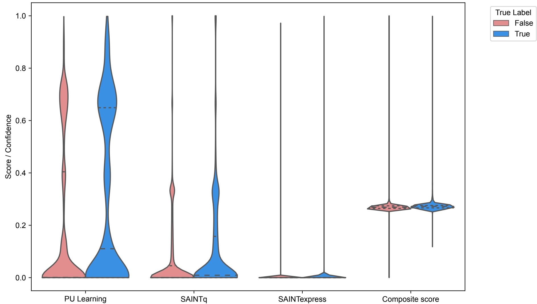
Score Distributions by Method and Label (Violin + Dots)
