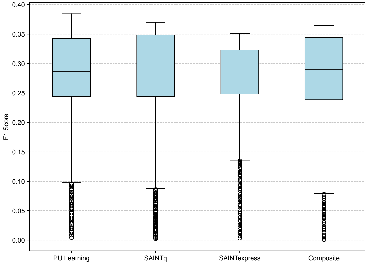
Distribution of F1 Scores Across Thresholds
