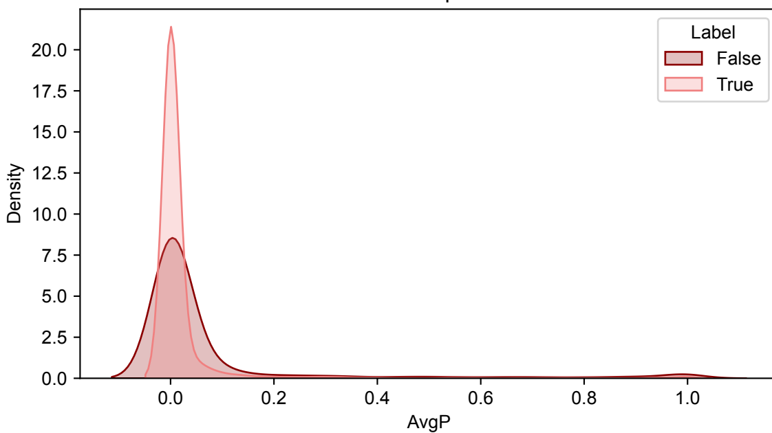
SAINTexpress
