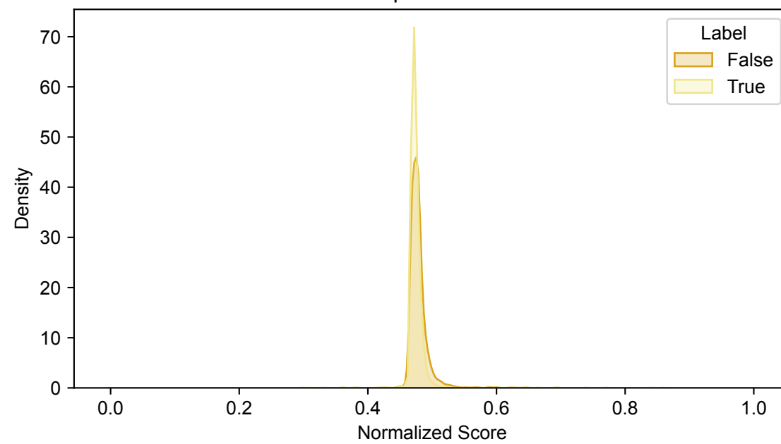
Composite Score
