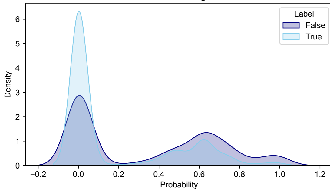
SAINTexpress
