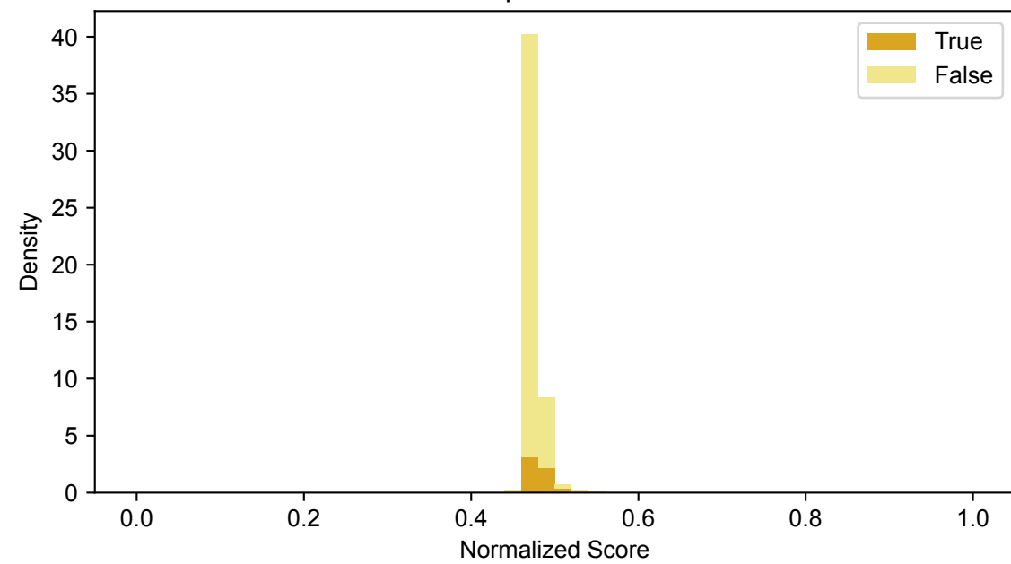
Composite Score
