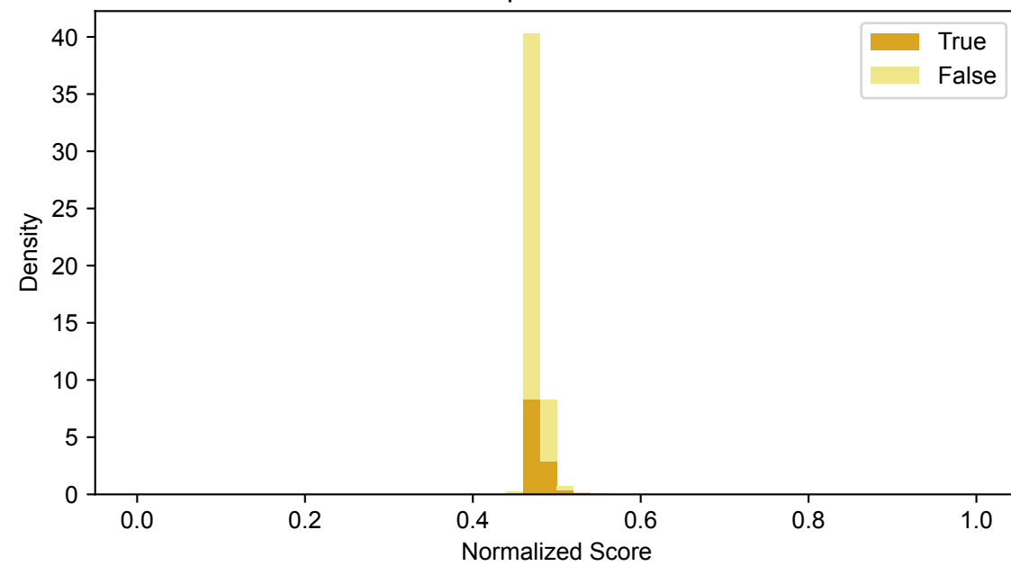
Composite Score
