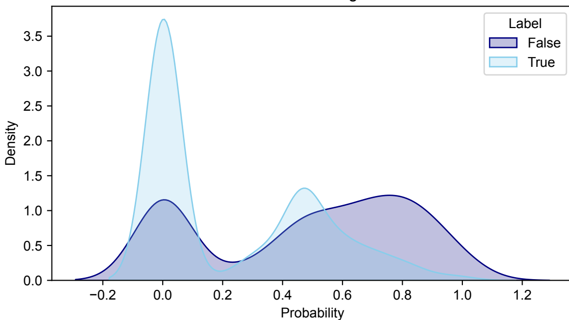
SAINTexpress
