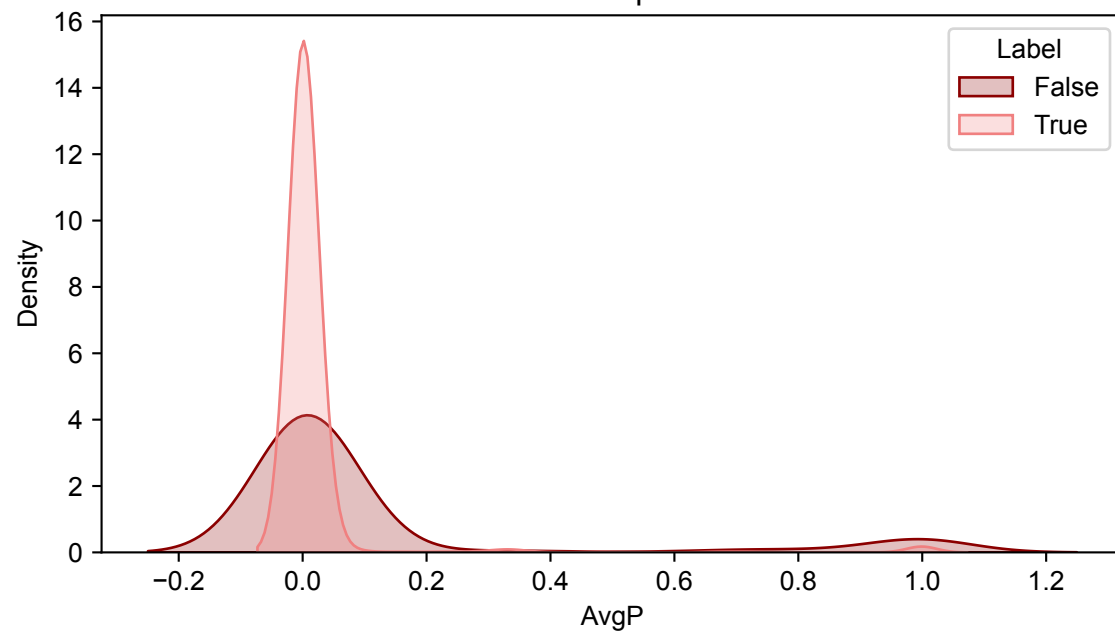
SAINTexpress
