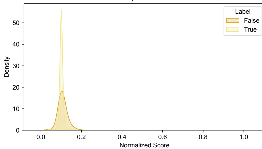
Composite Score
