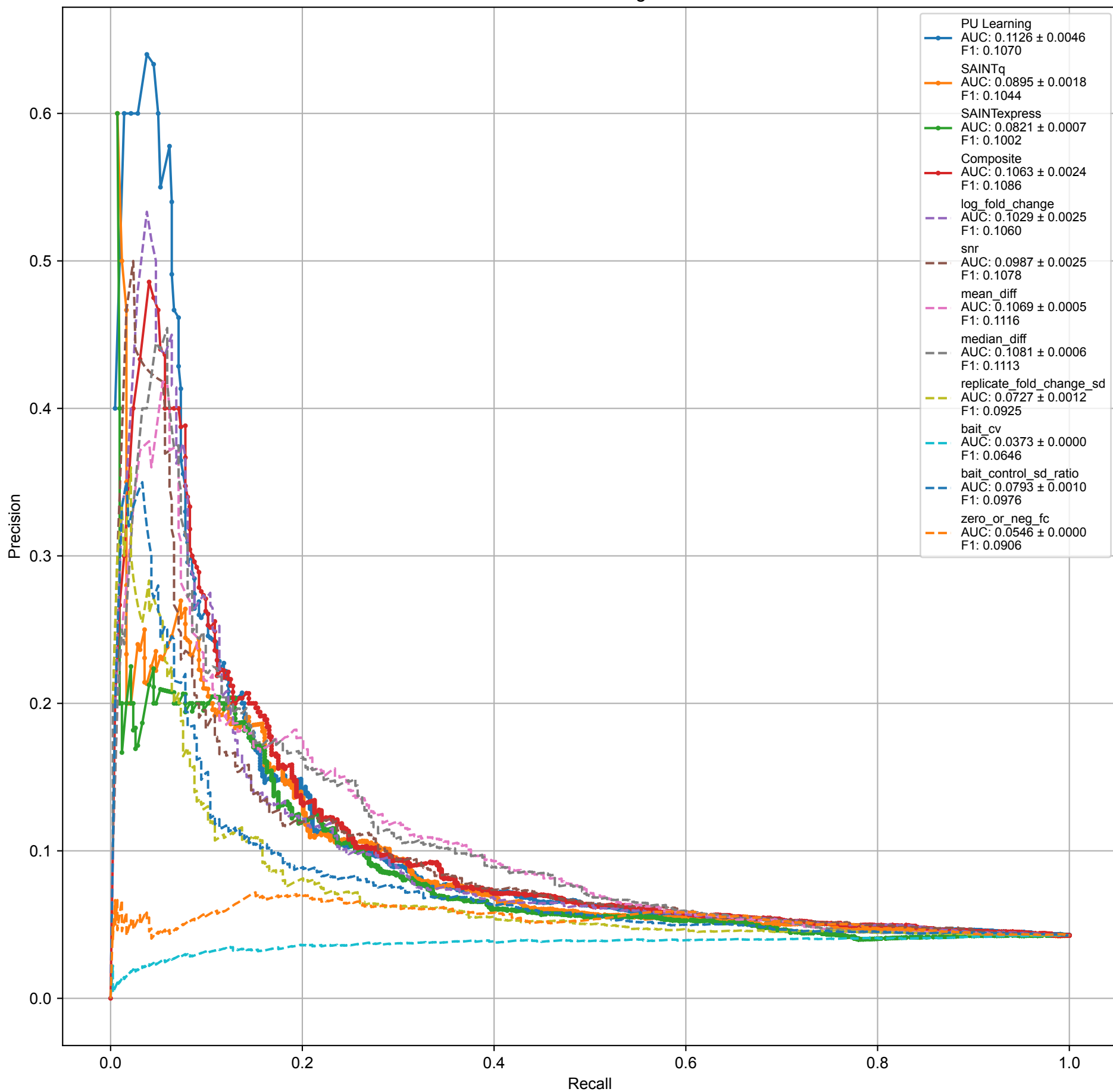
Precision–Recall Curve Including Individual Features
