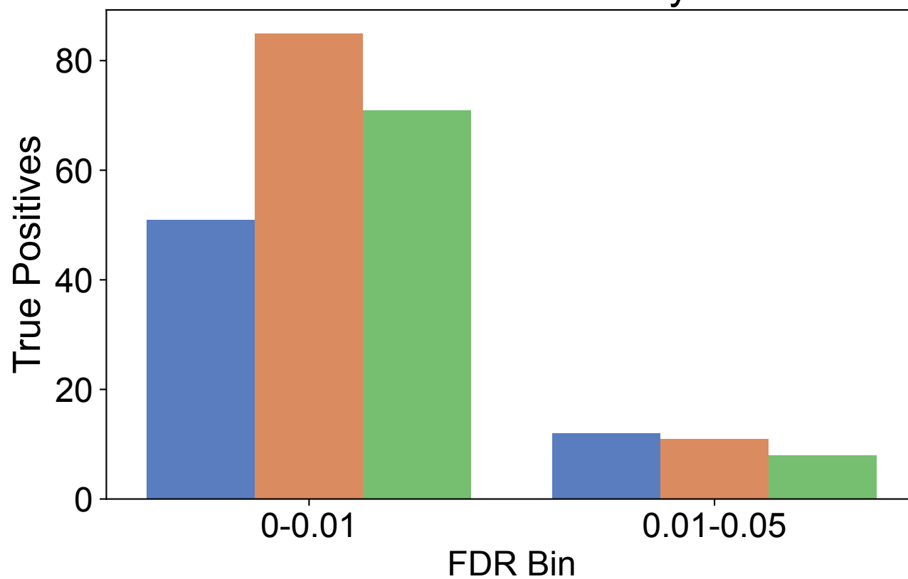
Number of True Positives by FDR Bin
