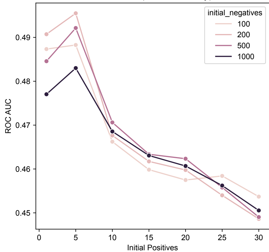
ROC AUC (Real vs Decoy)
