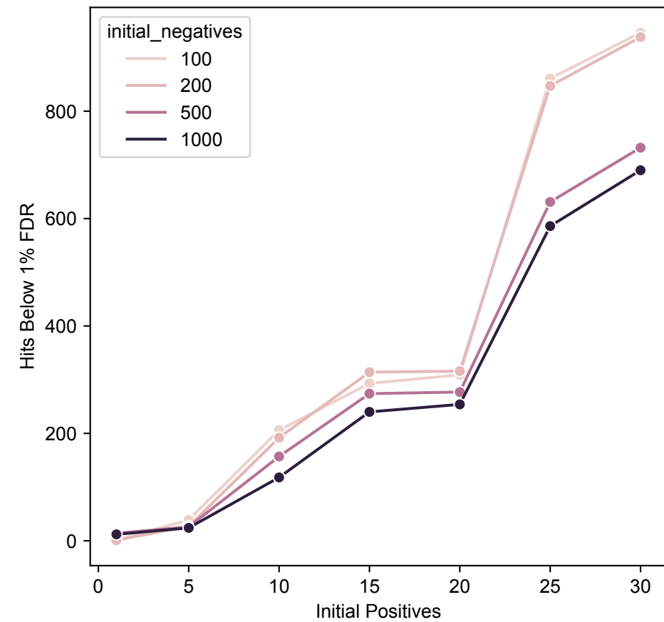
Hits Below 1% FDR
