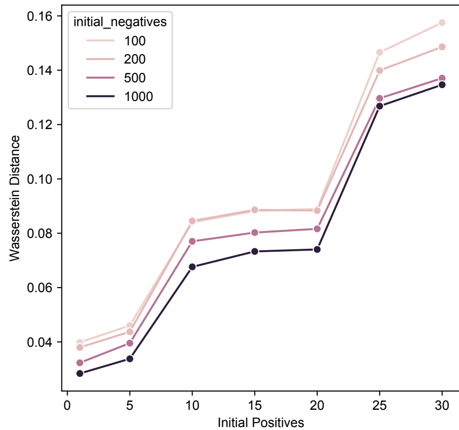
Wasserstein Distance
