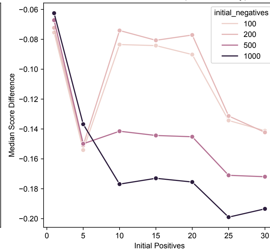
Median Score Difference (Real - Decoy)
