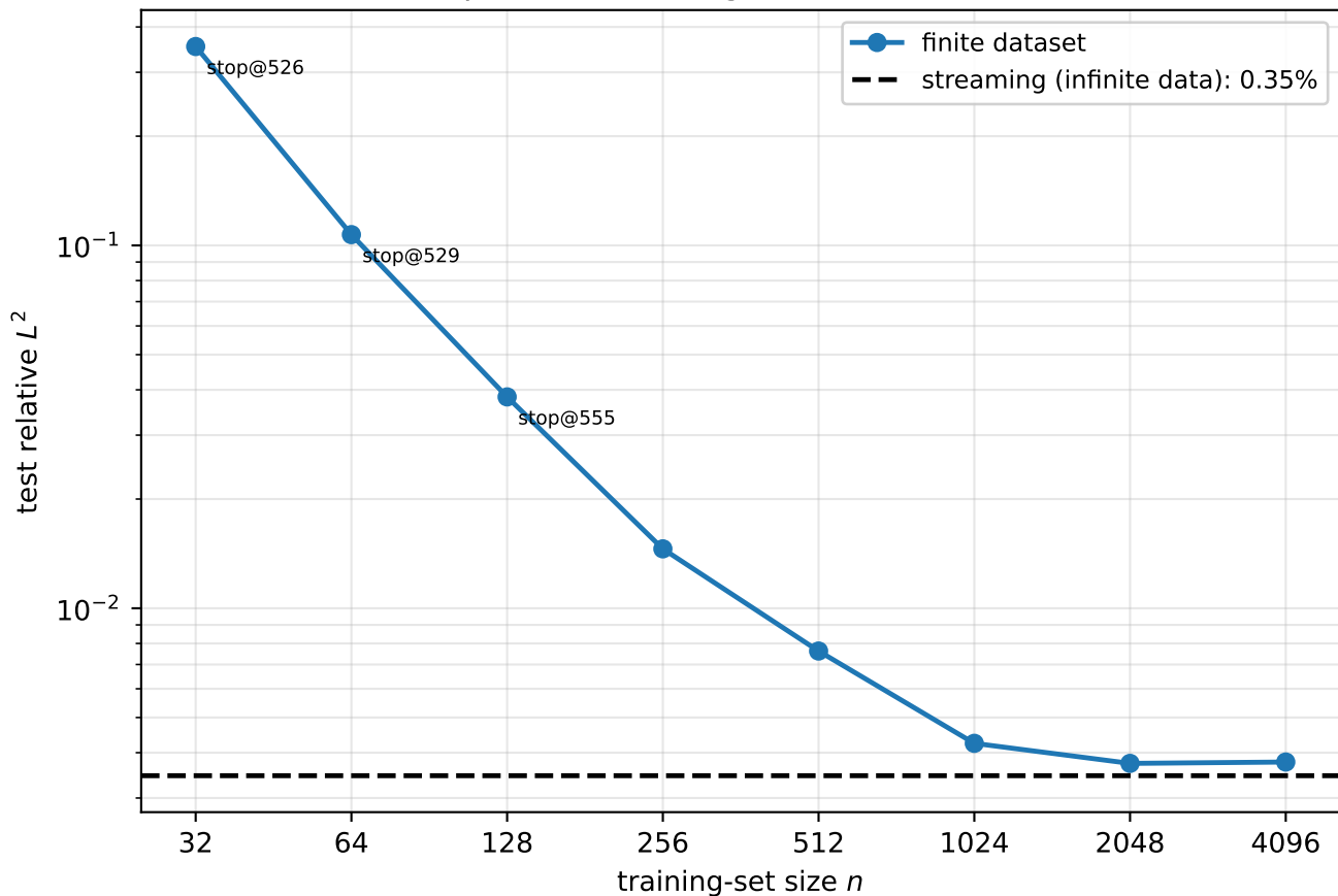
Fixed optimization budget: error vs dataset size
