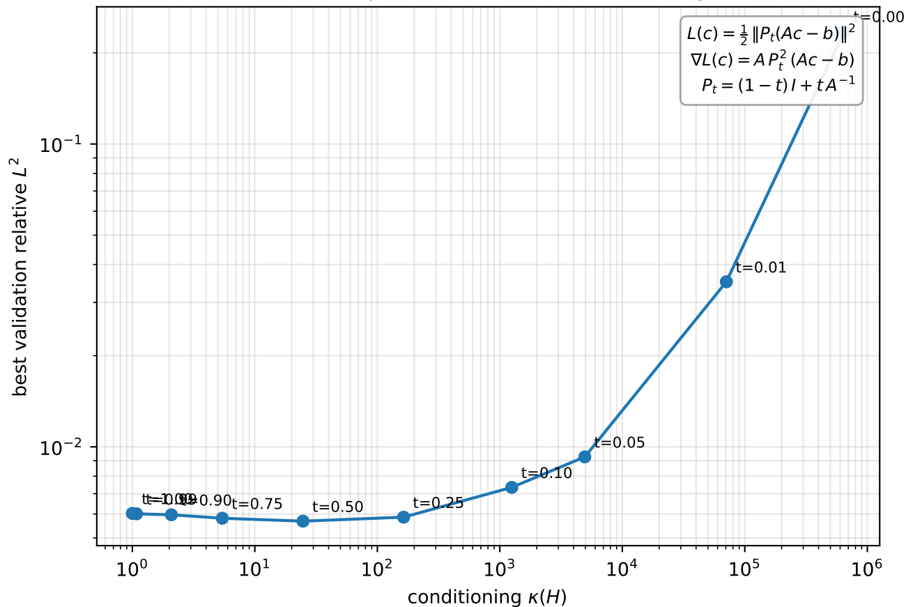
PLS collapse: final error vs conditioning
