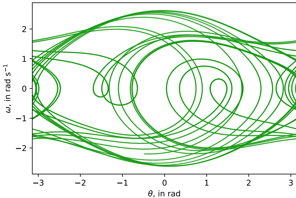
Phase portrait for A = 1.5
