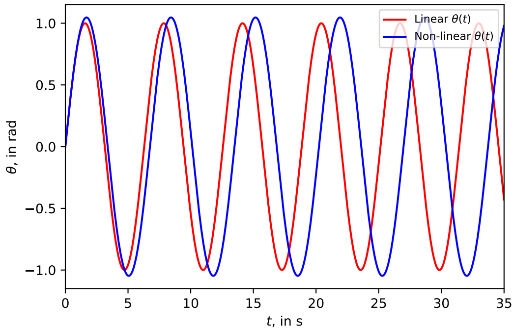
Plot of \theta(t) for \theta(0) = 0.0 , \omega(0) = 1.0
