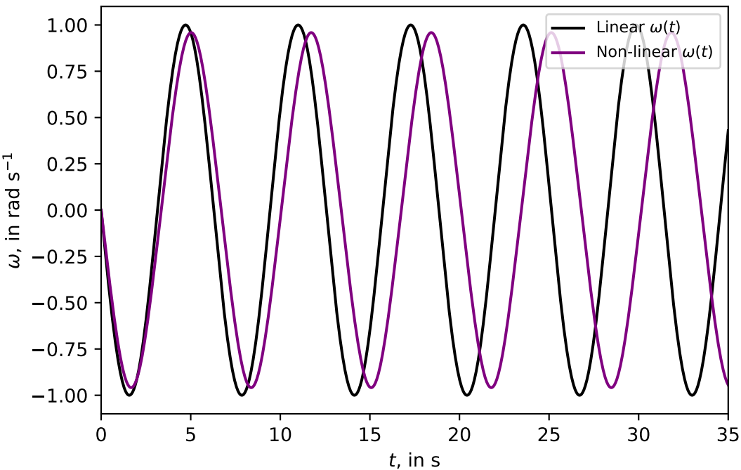
Plot of \omega(t) for \theta(0) = 1.0 , \omega(0) = 0.0
