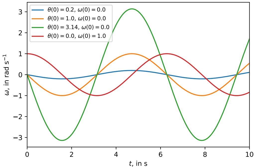
Plot of \omega(t) for various \theta(0) and \omega(0)
