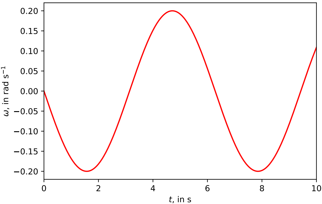
Plot of \omega(t) for \theta(0) = 0.2 and \omega(0) = 0.0
