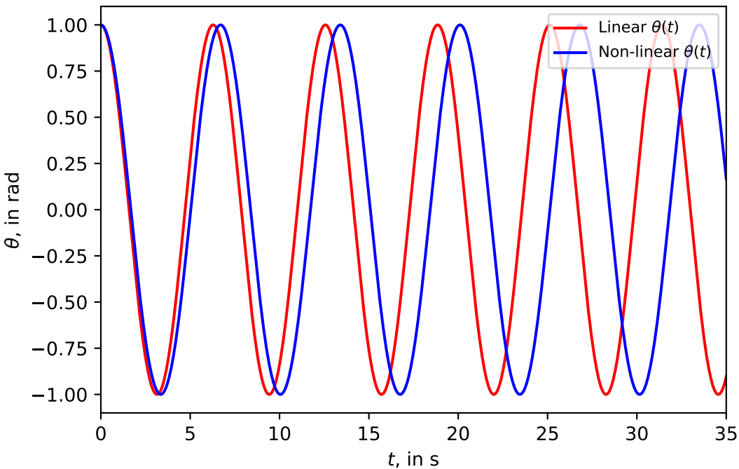
Plot of \theta(t) for \theta(0) = 1.0 , \omega(0) = 0.0
