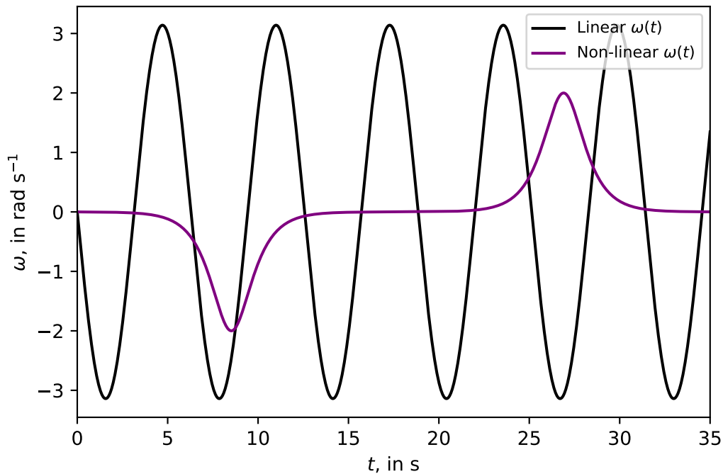
Plot of \omega(t) for \theta(0) = 3.14 , \omega(0) = 0.0
