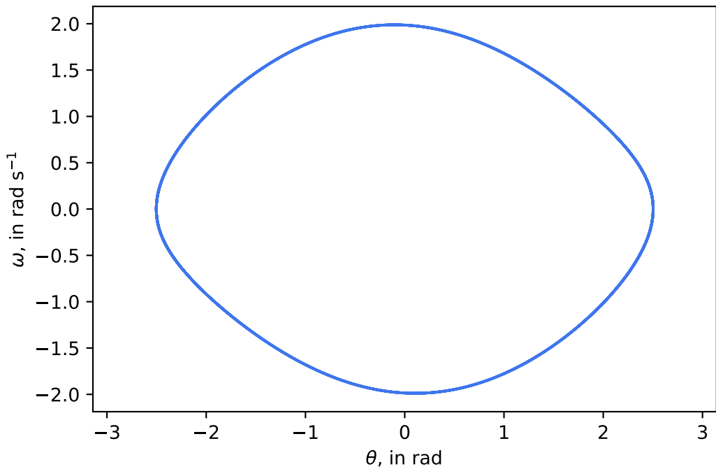
Phase portrait for A = 0.9
