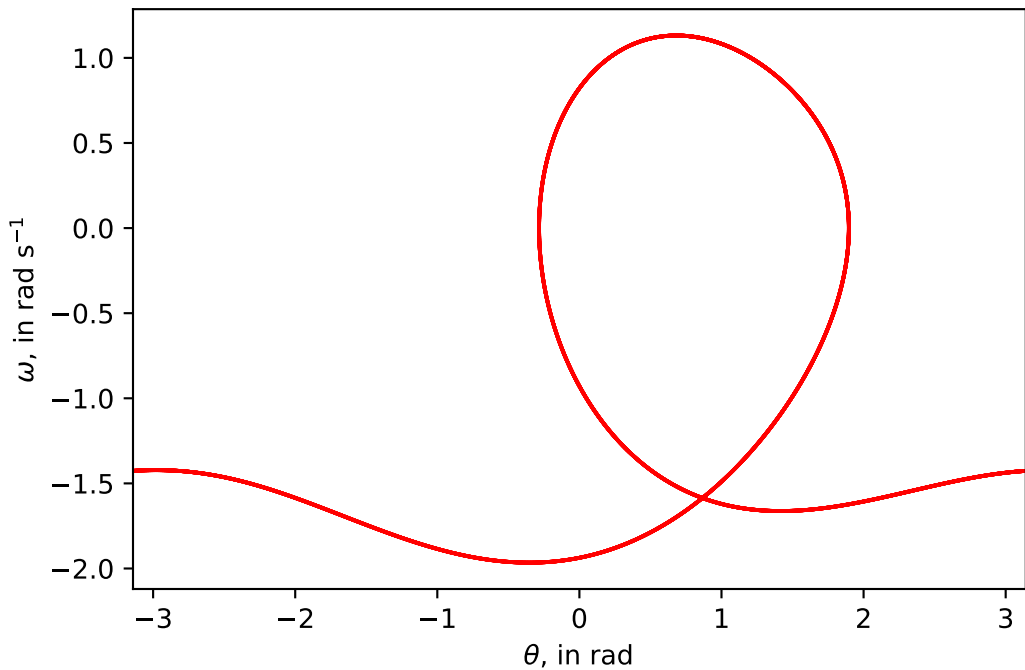
Phase portrait for A = 1.35
