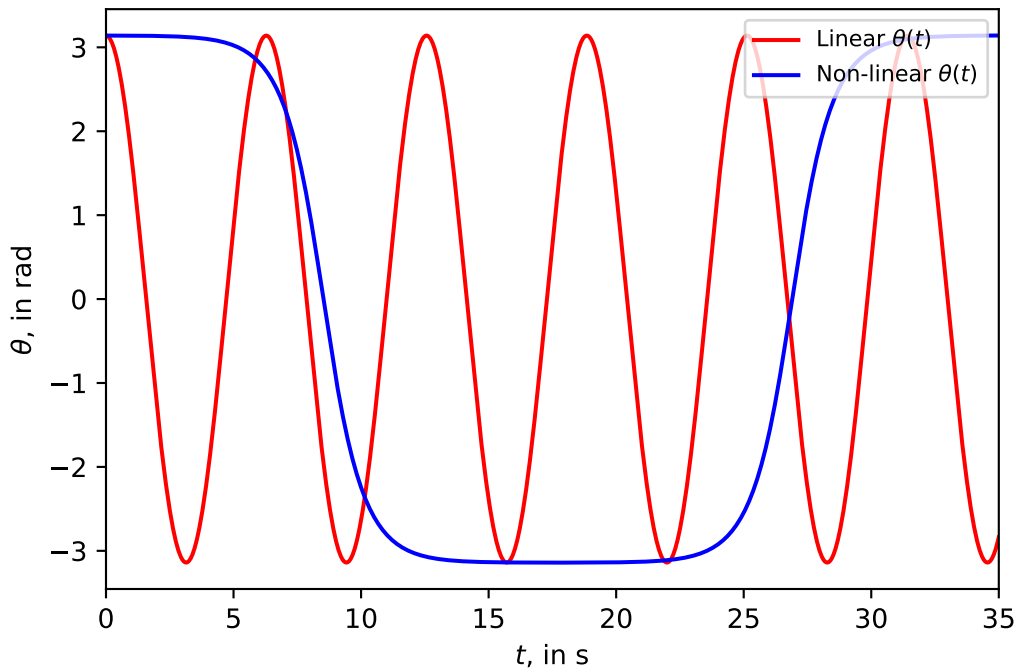
Plot of \theta(t) for \theta(0) = 3.14 , \omega(0) = 0.0
