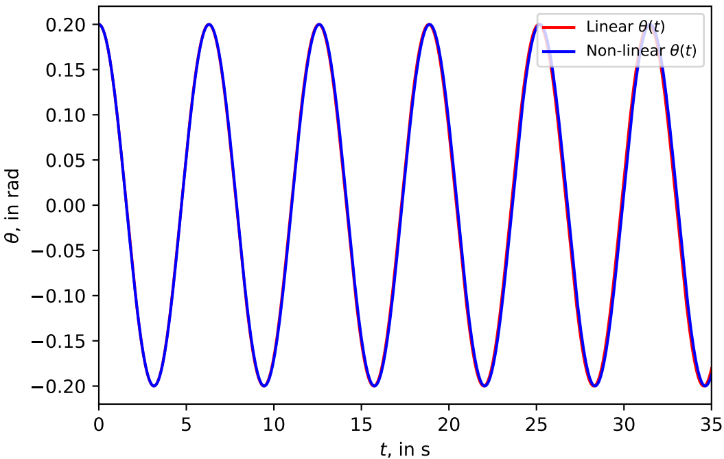
Plot of \theta(t) for \theta(0) = 0.2 , \omega(0) = 0.0
