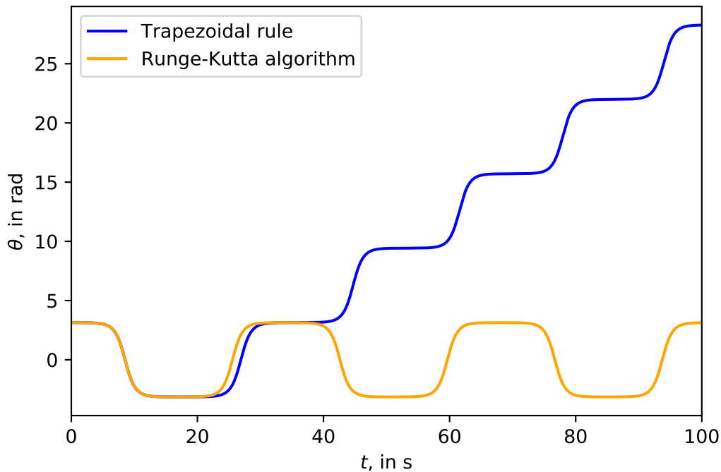
Plot of \theta(t) for \theta(0) = 3.14 , \omega(0) = 0.0
