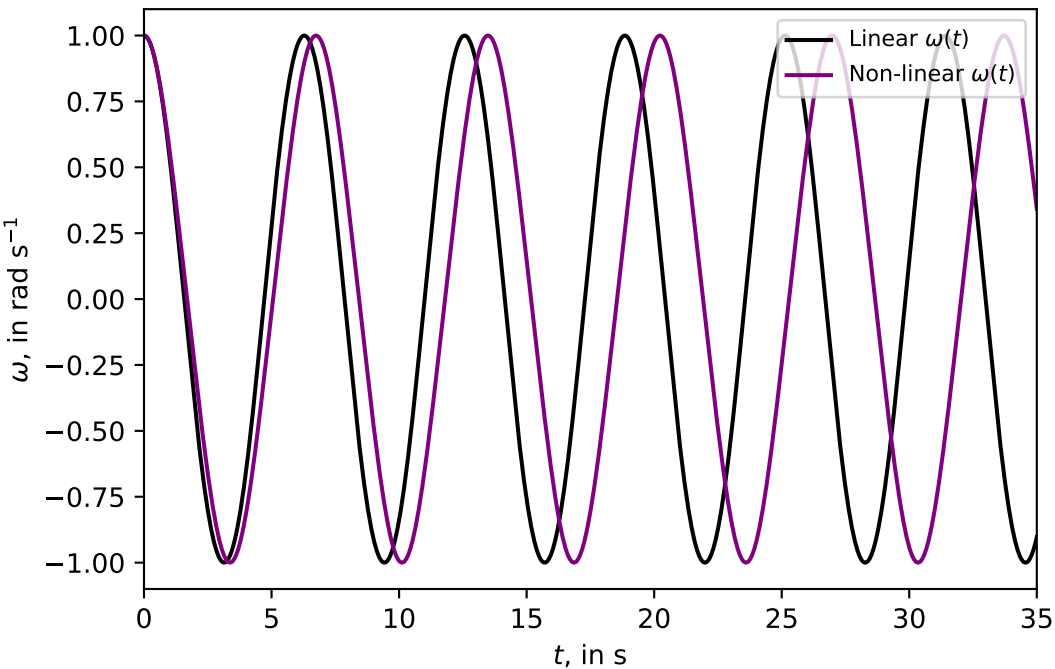
Plot of \omega(t) for \theta(0) = 0.0 , \omega(0) = 1.0
