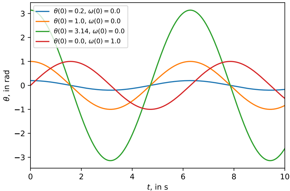
Plot of \theta(t) for various \theta(0) and \omega(0)
