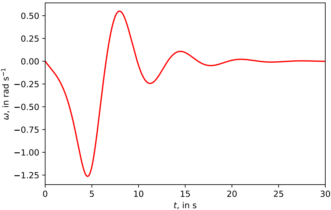
Plot of \omega(t) for \theta(0) = 3.0 , \omega(0) = 0.0
