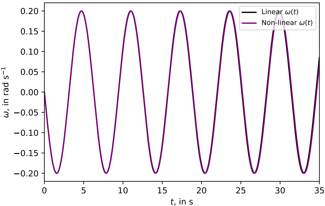
Plot of \omega(t) for \theta(0) = 0.2 , \omega(0) = 0.0
