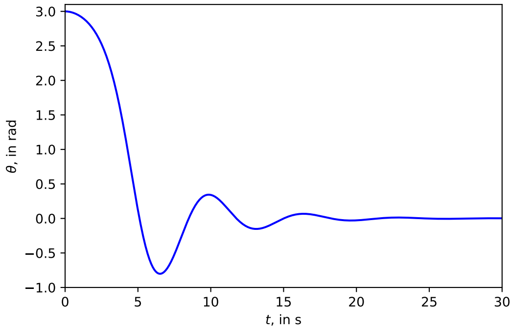
Plot of \theta(t) for \theta(0) = 3.0 , \omega(0) = 0.0
