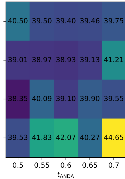
Minimum FID
