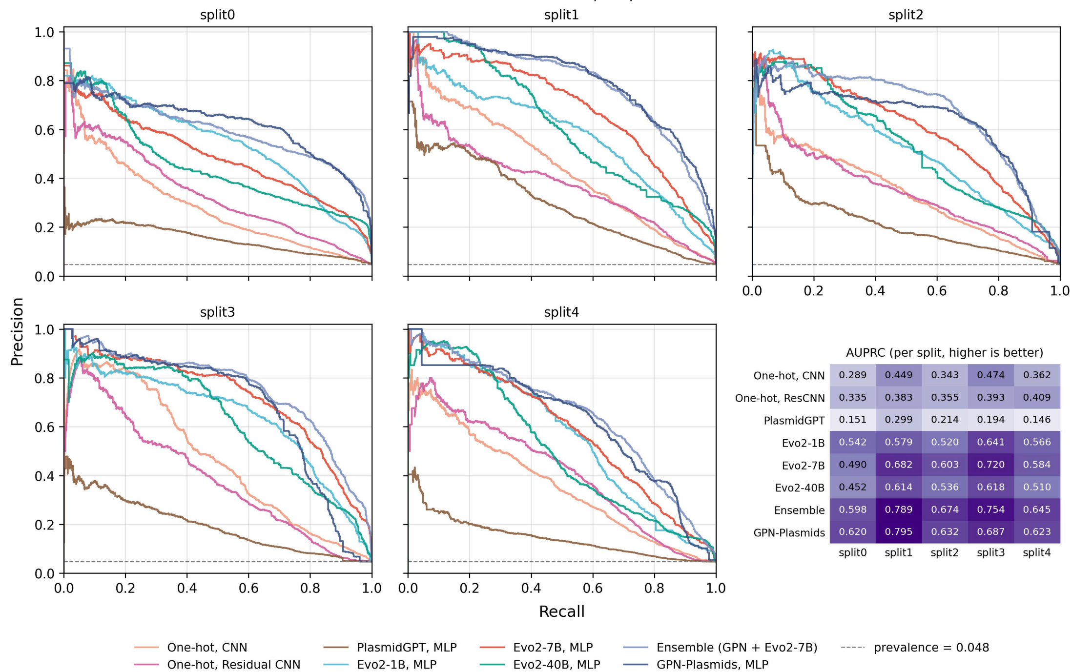
oriV window classification Precision-recall curves per split
