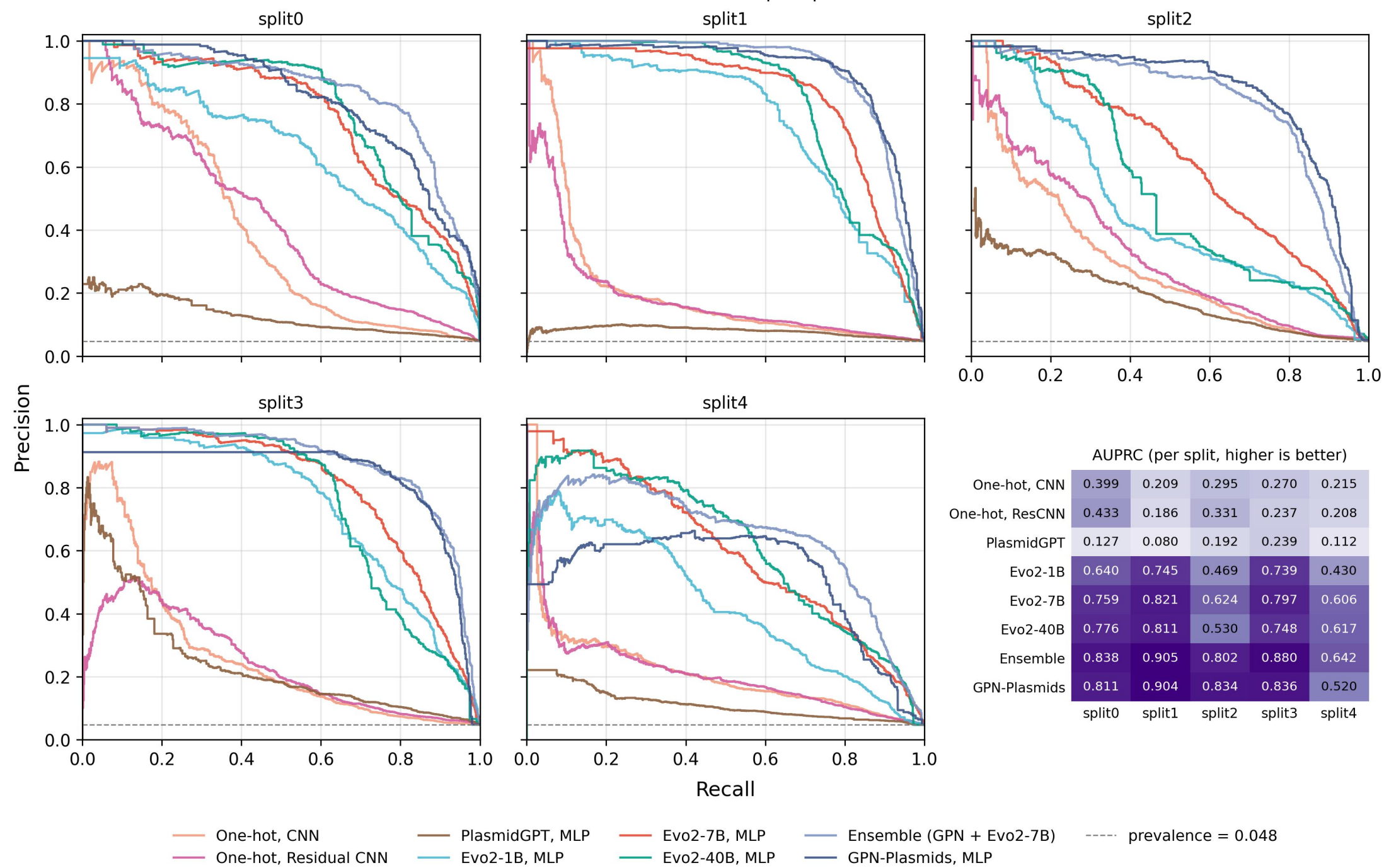
oriT window classification Precision-recall curves per split
