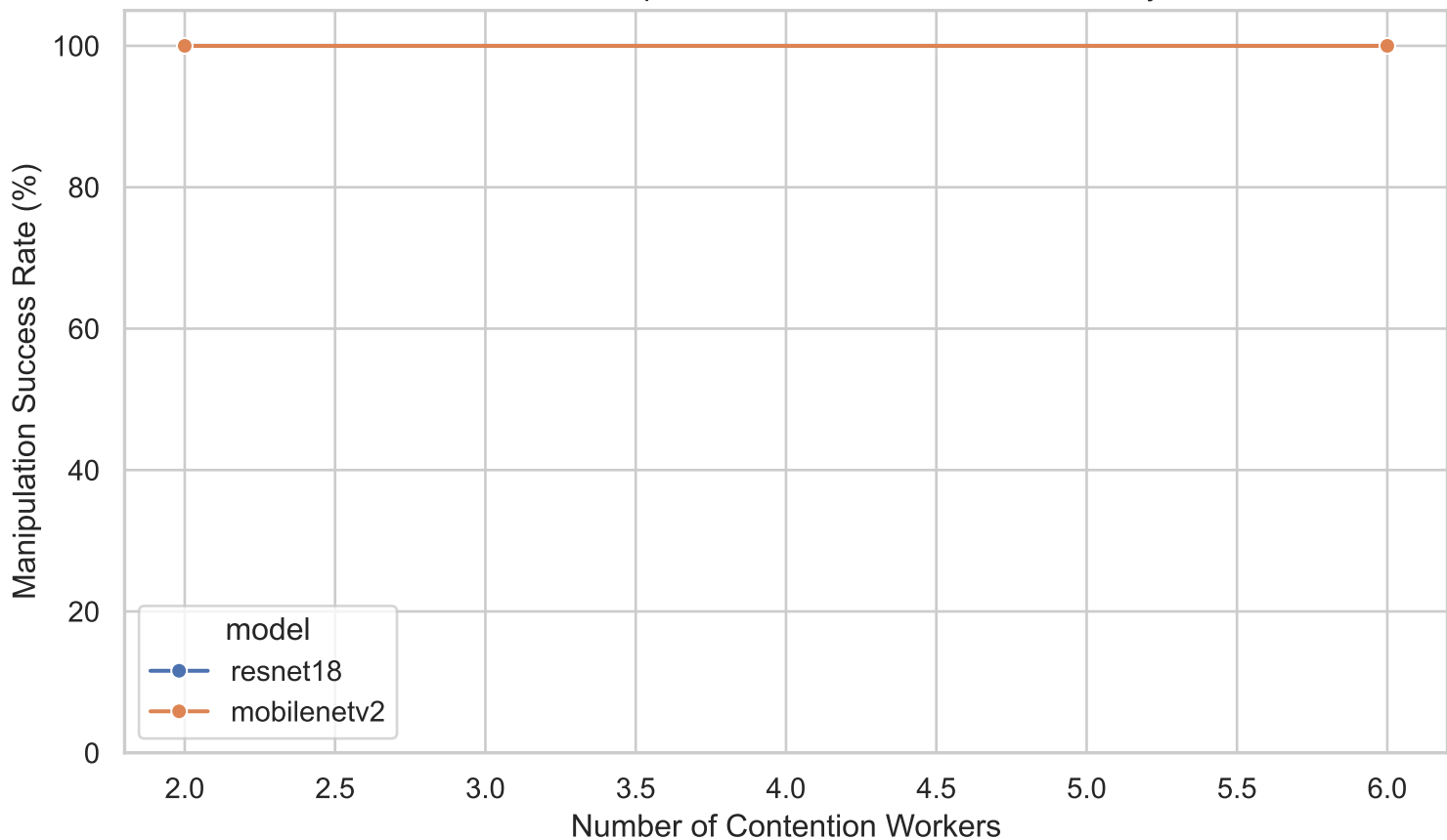
Adversarial Manipulation Rate vs. Contention Intensity
