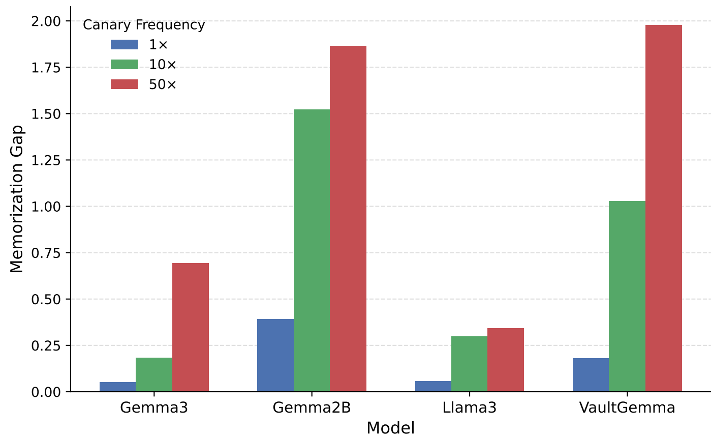
Frequency-Stratified Memorization Gaps at Baseline ( \epsilon = \infty )
