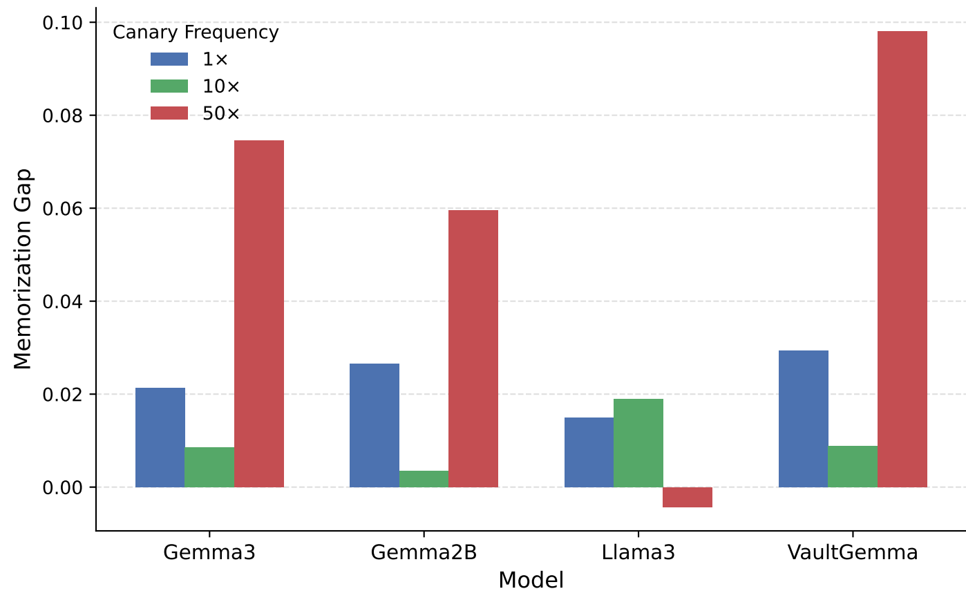
Frequency-Stratified Memorization Gaps ( \epsilon = 3 )
