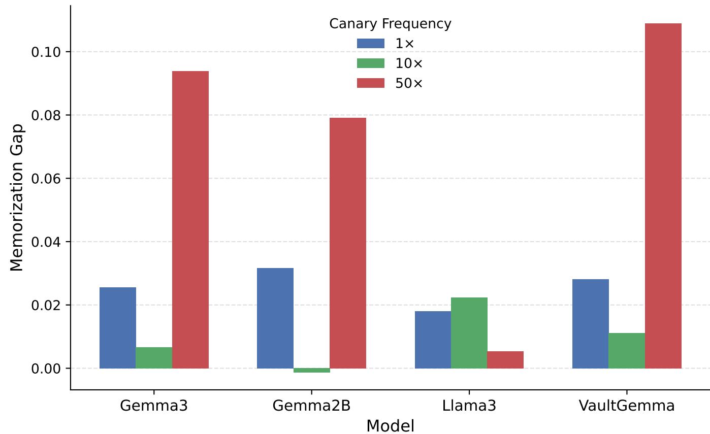
Frequency-Stratified Memorization Gaps ( \epsilon = 64 )
