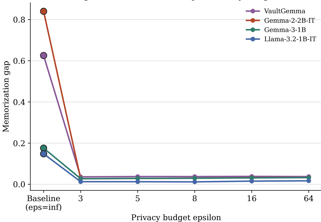
Figure 1: Memorization Gap vs Privacy Budget
