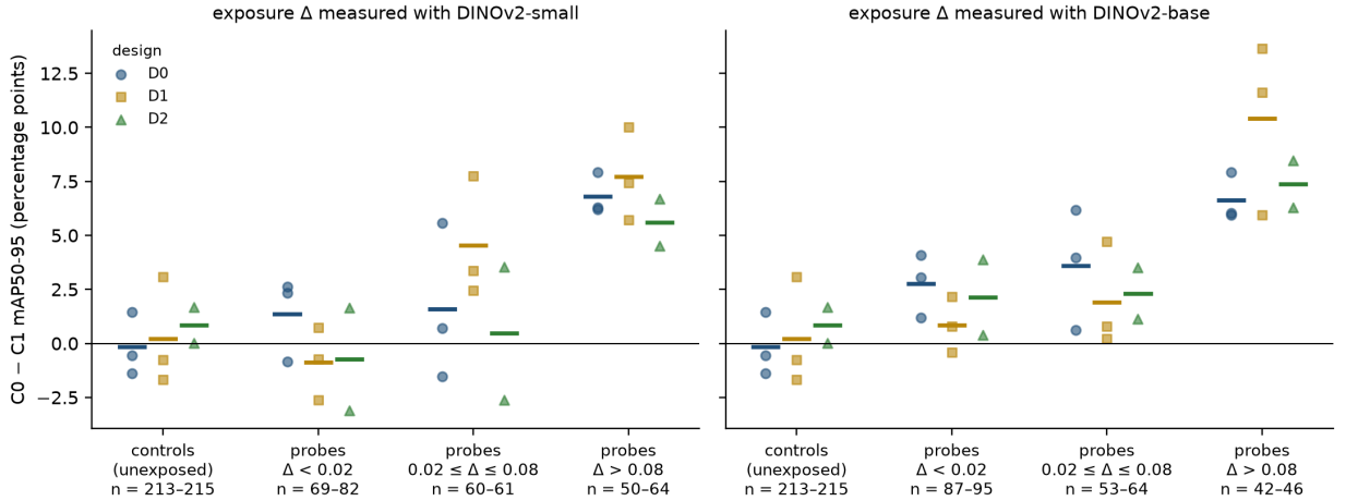
Markers: per-seed C0–C1 difference (8 matched seed pairs: D0×3, D1×3, D2×2); bars: mean over seeds of each design; no interval shown. n = test images per design. \Delta = max cosine to C0 training images – max cosine to C1 training images; bins fixed before the last three seed pairs were trained.
