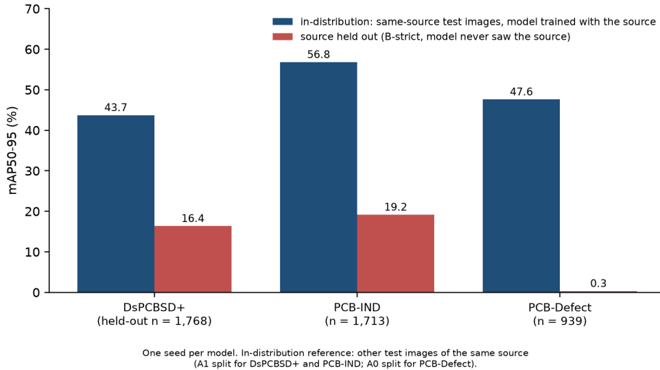
Figure 3: In-distribution vs source-held-out mAP50-95 (one seed per model).
