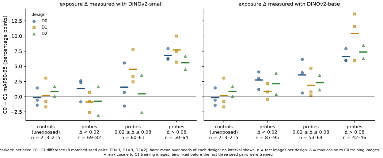
Figure 2: C0–C1 mAP50-95 by exposure stratum (left: DINOv2-small; right: DINOv2-base). Markers: per-seed differences (8 matched seed pairs); bars: design means; no interval drawn. n = test images per design.
