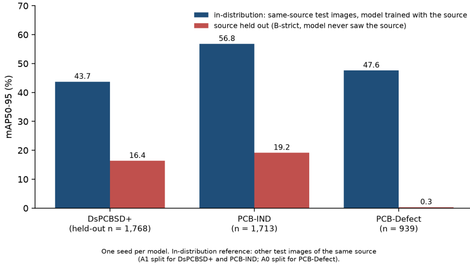
Figure 3: In-distribution vs source-held-out mAP50-95 (one seed per model).
