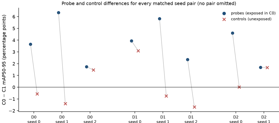
Figure 1: Probe and control C0–C1 differences for every matched seed pair.
