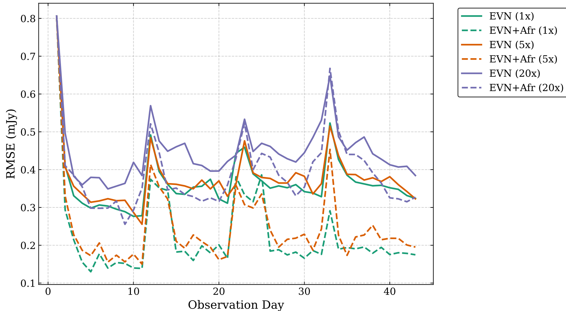
Global RMSE Evolution
