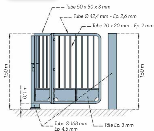
U oscillant Optimum+
