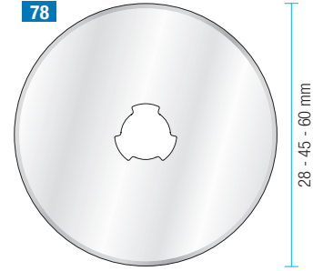
B657 Ölçüler / Dimensions: Ø28 x Th 0.30mm Ø45 x Th 0.30mm Ø60 x Th 0.35mm
