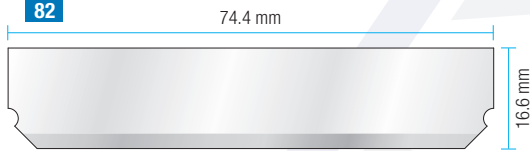
B644 74.4 x 16.6 x 0.884 mm Tunsten Alaşımli Çelik / Tungsten Alloyed Steel TiN Kaplama / TiN Coated Solid Tungsten Carbide
