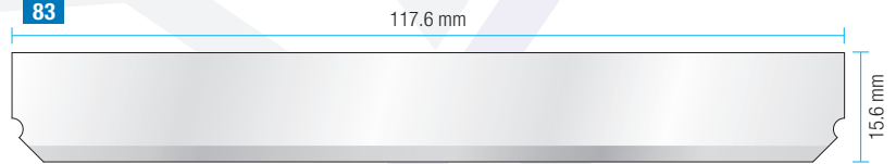
B645 117.6 x 15.6 x 0.884 mm Tunsten Alaşımli Çelik / Tungsten Alloyed Steel TiN Kaplama / TiN Coated Solid Tungsten Carbide
