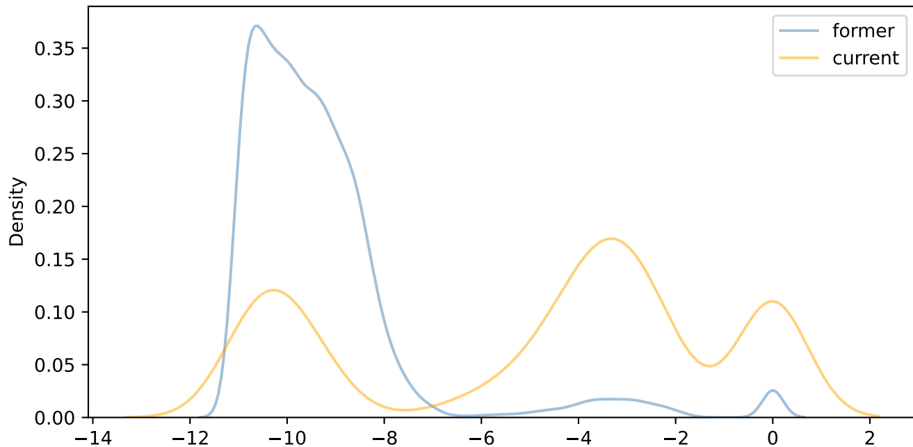
Distributions of \log(\text{partial-correlation}) values where greater than zero
