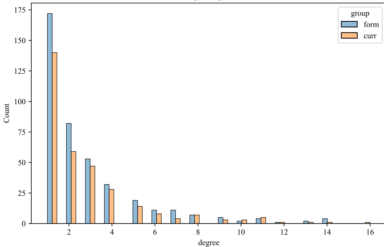
Graph Degrees
