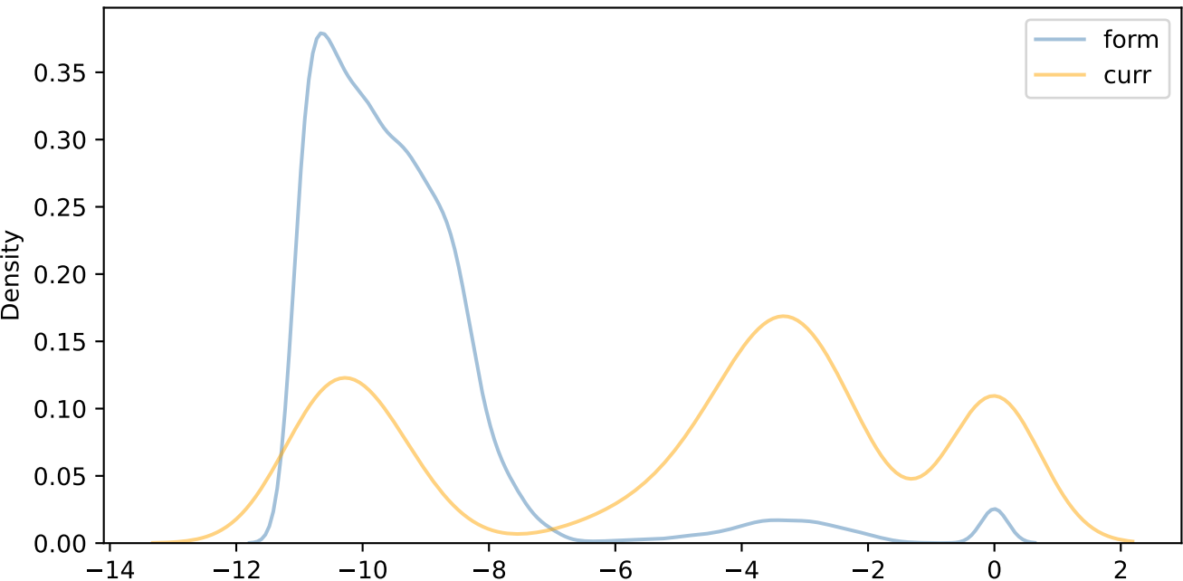
Distributions of \log(\text{partial-correlation} > 0)
