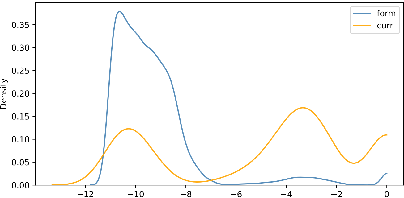
Distributions of \log(\text{abs}(\text{partial-correlation}) > 0) ( \tau = 0.046 )
