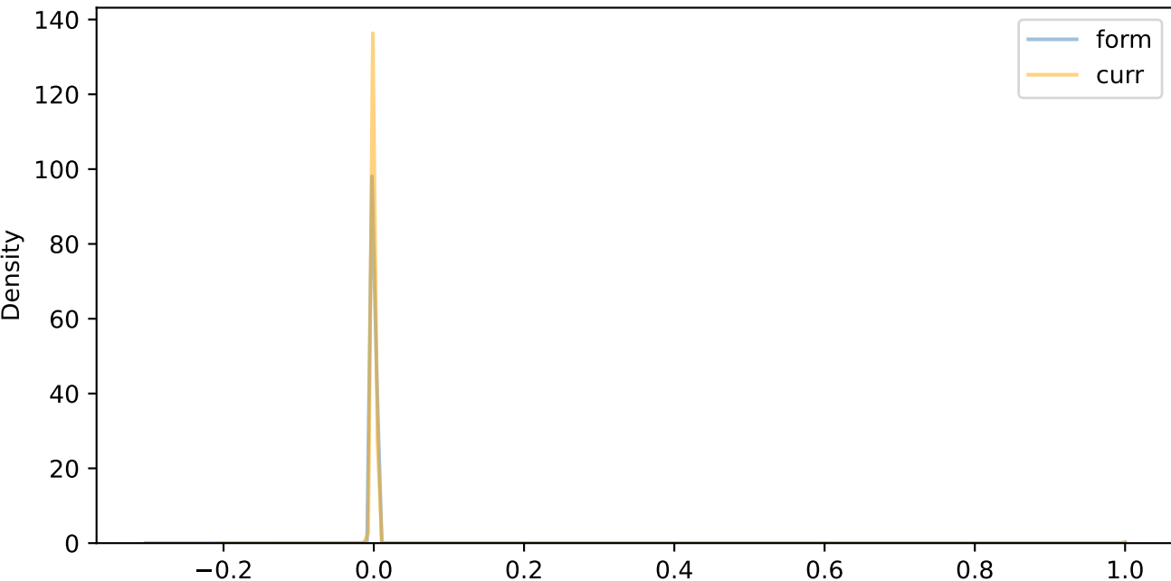
Distributions of partial-correlation ( \tau = 0.046 )
