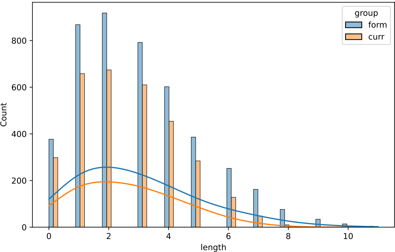
Shortest Path Lengths
